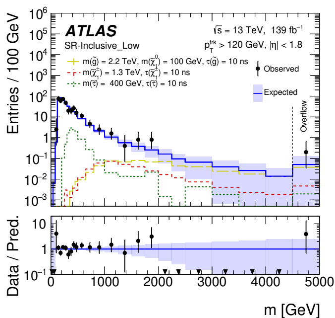
(a) SR-Inclusive_Low
