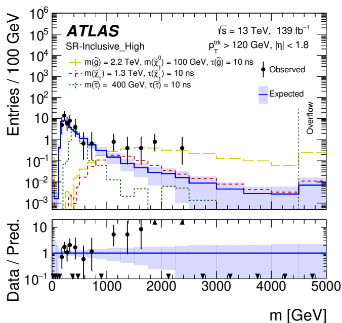
(b) SR-Inclusive_High
