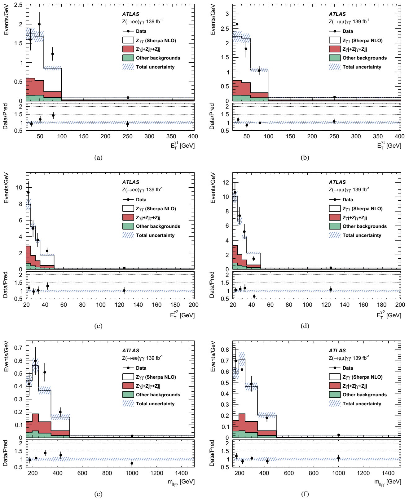
Fig. 3 The detector-level distributions in data compared with signal-plus-background predictions in the electron and muon channels for a, b E_T^{\gamma 1} , c, d E_T^{\gamma 2} and e, f m_{ll\gamma\gamma} . The lower panels show the ratio of the data to the total prediction
