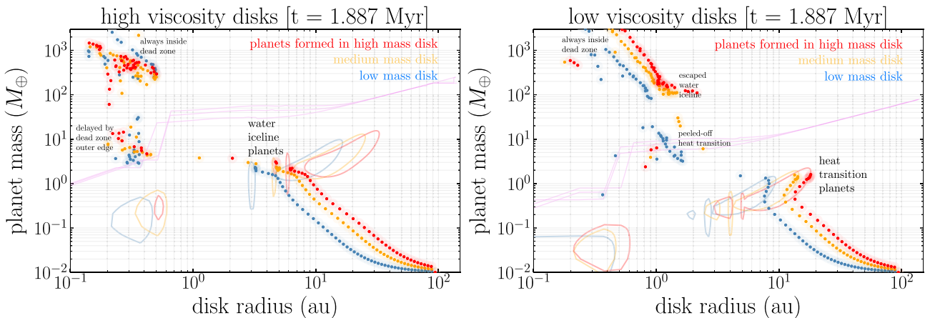
Figure 6. Planet masses and semimajor axes at the age of HL Tau. Results from all six of our formation scenarios: high-mass (red), medium-mass (orange) and low-mass (blue) HL Tau discs, at two levels of viscosity (broadly, \alpha = 10^{-3} and \alpha = 10^{-4} ; see top panel of Fig. 1). Each dot (planet) is surrounded by a faded circle simply to give the reader a sense of number density. As always, results for the high viscosity discs are shown on the left, and low viscosity on the right. For reference, and to put the planets’ locations in the context of the torque maps, we overlay the gas gap-opening mass in pink (equation 21), and the three contours of zero net torque in colours corresponding to disc mass (see also Figs 2 and 4). We identify planets trapped at the water iceline in the high viscosity discs as ‘water iceline planets,’ and those trapped outside the heat transition in the low viscosity discs as ‘heat transition planets’ (see Fig. 7’s movie).
