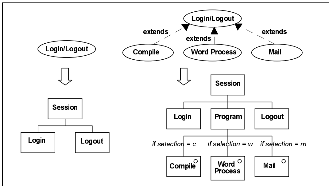
Figure 1: Jacobson's extends relationship translated into a structure chart
