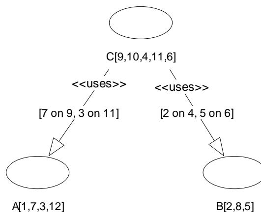
Figure 1. Multiple uses-relation between use cases
