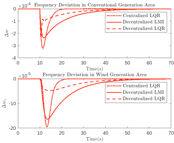
Fig. 2. Frequency response to a load disturbance of \Delta P_L = 0.01 p. u. (20 MW) in CA1 at t = 10 s.
