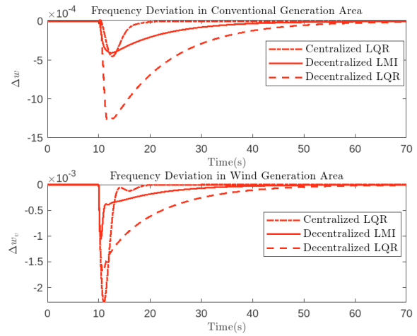
Fig. 5. Frequency response to a load disturbance of \Delta P_L = 0.01 p. u. (20 MW) in CA2 at t = 10 s.
