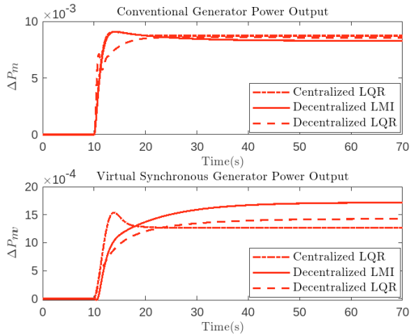
Fig. 3. Power outputs of generators during a load disturbance of \Delta P_L = 0.01 p. u. (20 MW) in CA1 at t = 10 s.
