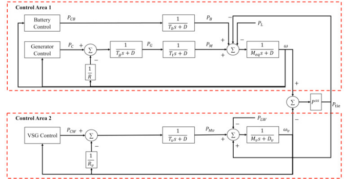
Fig. 1. The hybrid power system incorporating conventional generation, battery storage and wind generation, and the proposed decentralized control architecture.
