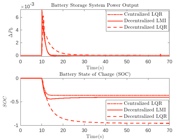
Fig. 4. BESS power output and state of charge during a load disturbance \Delta P_L = 0.01 p. u. (20 MW) in CA1 at t = 10 s.
