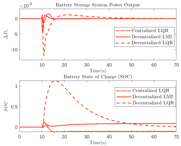
Fig. 7. BESS power output and state of charge during a load disturbance \Delta P_L = 0.01 p. u. (20 MW) in CA2 at t = 10 s.
