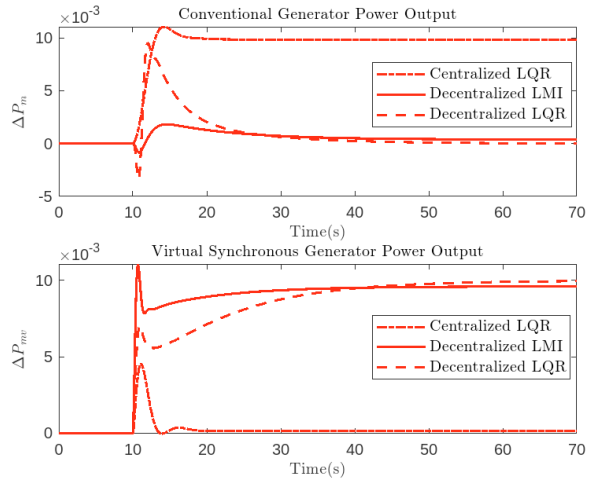
Fig. 6. Power outputs of generators during a load disturbance of \Delta P_L = 0.01 p. u. (20 MW) in CA2 at t = 10 s.
