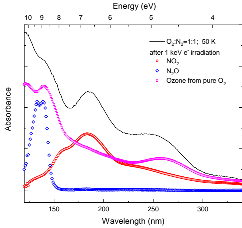
Fig. 7. VUV absorbance spectrum (120–340 nm) of a frozen mixture \text{O}_2:\text{N}_2 = 1:1 obtained after electron bombardment and annealing to 50 K (solid black line) is compared to VUV spectra of \text{O}_3 at 50 K formed after electron irradiation of pure \text{O}_2 at 22 K (magenta squares), pure deposited \text{NO}_2 (red circles), and \text{N}_2\text{O} ices at 22 K (blue diamonds).
