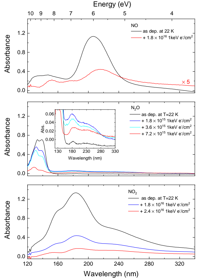
Fig. 8. VUV absorbance spectra (120–340 nm) of pure \text{NO} (top panel), \text{N}_2\text{O} (middle panel), and \text{NO}_2 (bottom panel) ices as deposited at 22 K (solid black lines) and after exposure to 1 keV electrons.
