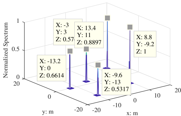
Fig. 5: Localization results for five targets with six sub-arrays (20dB SNR, 500 snapshots).
