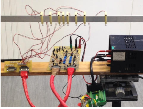
(a) A co-prime microphone array system
