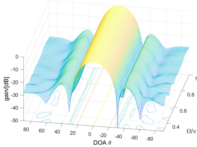
Fig. 1: A design example for a frequency invariant beamformer.
