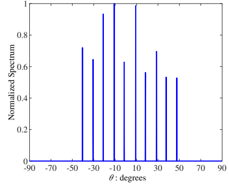
(b) Estimation result for 10 sources
