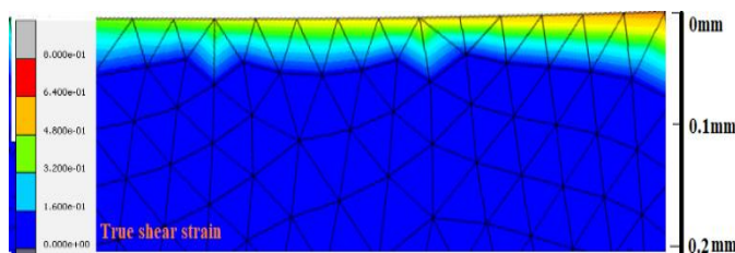
Fig. 7. True shear strain map for the surface machined (minimum element size 0.04mm)
