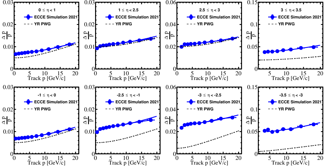
Figure 8: ECCE pion track momentum resolution (data points) with the EIC YR PWG requirements for the tracker indicated by the dashed lines. Note that the ECCE performance simulations take into account materials for readout and services. The impact of these can be observed most clearly in the bins covering the barrel/barrel endcap transition regions. As an integrated EIC detector with all subsystems operating in a complementary way, ECCE achieves the EIC physics goals.
