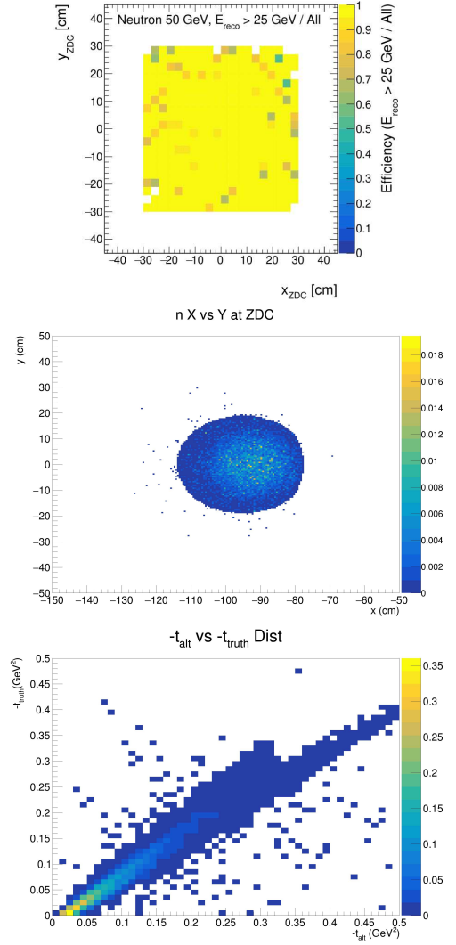
Figure 26: (top) ZDC detection efficiency for neutrons in its local coordinate system. (middle) Detection distribution of neutron hits in the ZDC for meson structure function processes without the beam pipe blocking contribution. z -axis reflects the normalized yield. (bottom) Reconstructed t versus true t , where t is reconstructed as from the baryon information, t_{alt} = (p_p - p_n)^2 , which is reliable with a resolution of < 0.025 GeV 2 .
