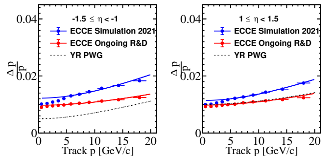
Figure 10: The momentum dependence of the tracker momentum resolution for the ECCE reference tracker design (ECCE Simulation, blue solid circles) and for the projective mechanical support design of the ECCE ongoing project R&D that will continue after the proposal (red solid circles). The latter shows a reduction of the impact of readout and services on the tracking resolution. Note that the backward region (left panel) relies on the EM calorimeter, and thus a resolution larger than the EIC YR PWG requirement is acceptable.
