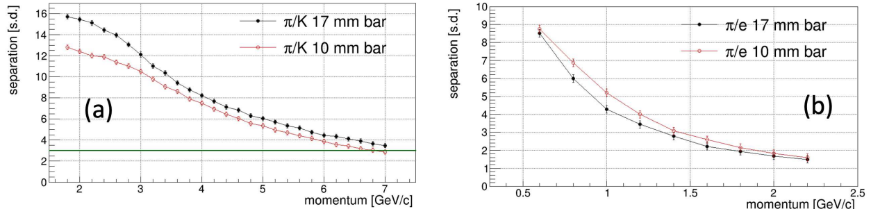
FIG. 29. Expected performance of the hpDIRC: Separation power ( n\sigma ) for \pi/K (a) and e/\pi (b) for two different bar thickness values as a function of the particle momentum. Results are based on a standalone Geant4 simulation and shown for a polar angle of 30^\circ .
