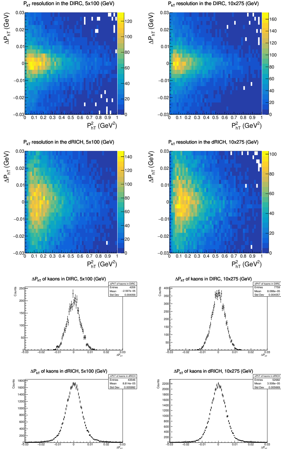
FIG. 9. Resolution in the kaon's transverse momentum (w.r.t. the virtual photon) for kaons in the DIRC or dRICH for the 5×100 (left column) and 10×275 (right column) beam-energy settings. Top two rows depict the resolution vs. transverse kaon momentum; the bottom two rows show the canvas integrating over transverse momentum. The Electron Method is used for reconstruction of the DIS kinematics, and the CORE resolution is again simulated with DELPHES.
