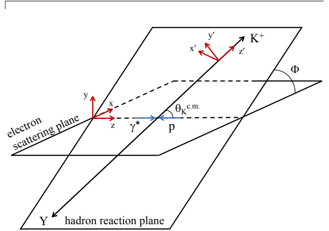
FIG. 1. Kinematics for K^+Y electroproduction defining the c.m. angles and coordinate systems used to express the formalism and to present the polarization components extracted in the analysis.
