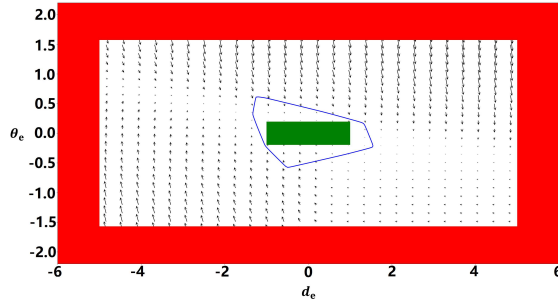
Fig. 8. NN controller learned and verified for Example 1 with larger safety margin: \varepsilon_1 = 0.02, \varepsilon_2 = 0.8, \varepsilon_3 = 0.01, \varepsilon_4 = 0.05 ; the inner (green) and outer (red) shaded areas are the initial and unsafe regions, black arrows in the white area are the closed-loop vector fields \mathbf{f}(\mathbf{x}, \mathcal{N}_c(\mathbf{x})) , and the blue curve surrounding the inner shaded box is the zero-level set of \mathcal{N}_b
