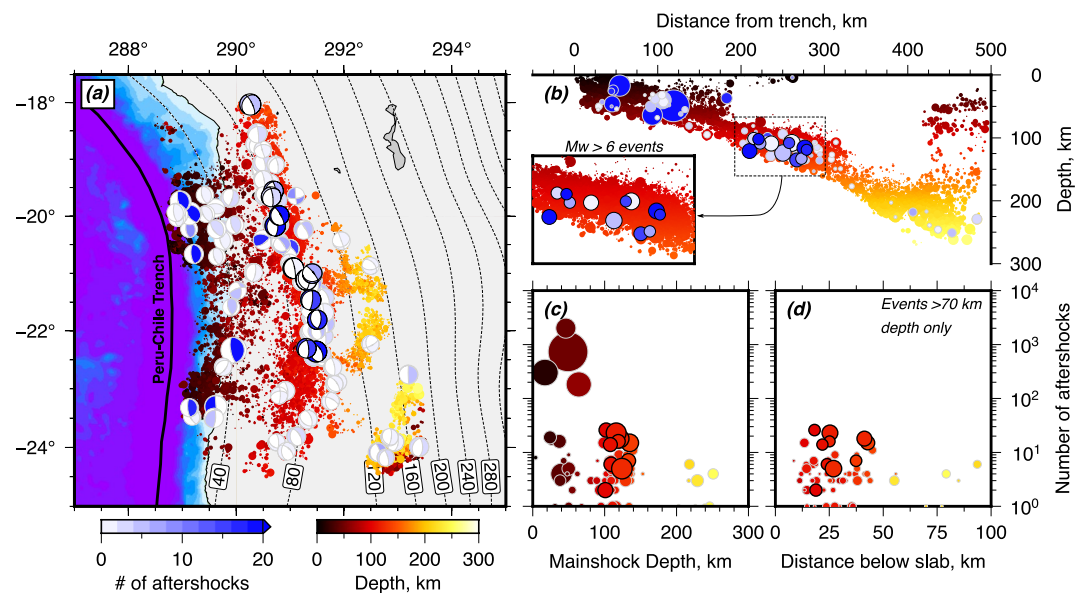
Figure 2. Aftershock productivity of moderate-magnitude earthquakes in northern Chile using the IPOC catalog of Sippl et al. (2018). (a) Map of the spatial distribution of the seismicity overlain with the focal mechanisms of the mainshocks taken from the gCMT catalog. The focal mechanisms are colored by the number of counted aftershocks. Mainshocks that are M_w 6.0–6.5 and at depths \geq 70 km are highlighted by a black outline. Slab contours are from Slab 2.0 (Hayes et al., 2018). (b) Cross-section through the IPOC seismicity overlain by the mainshocks shown as blue circles. Mainshocks are scaled by magnitude. (c) Aftershock productivity as a function of mainshock depth for mainshocks across all depths. (d) Aftershock productivity as a function of depth below the slab surface for mainshocks with hypocentral depths > 70 km only.
