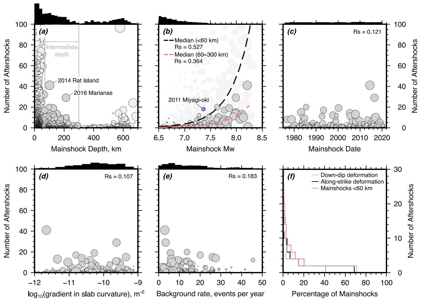
Figure 1. Aftershock productivity for earthquakes in the gCMT catalog with M_w \geq 6.5 . (a) Aftershock productivity as a function of the mainshock depth. Intermediate-depth earthquakes (60–300 km) are shown in dark gray. The histogram of the logarithm of mainshock frequency with depth is shown above. (b) Aftershock productivity as a function of mainshock magnitude. Intermediate-depth earthquakes are shown in dark gray with black outline, whilst earthquakes with hypocentral depths <60 km are shown as light gray circles. The median aftershock productivity scaling is shown for shallow and intermediate-depth mainshocks. R_s is the Spearman's Correlation Coefficient. (c) Aftershock productivity as a function of mainshock date, (d) the gradient in the down-dip curvature of the slab at the centroid location computed from Slab 2.0 (Hayes et al., 2018), and (e) the background seismicity rate within 50 km horizontal distance and \pm 30 km depth difference from the mainshock hypocenter. (f) Histogram of aftershock productivity for mainshocks that accommodate either along-strike or down-dip deformation of the slab. The red histogram shows the productivity for shallow earthquakes with hypocentral depths <60 km.
