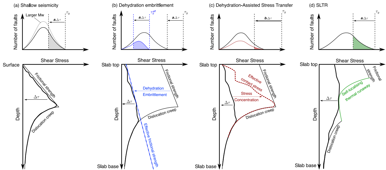
Figure 9. Sketch of the effect of stress transfer from an earthquake stress drop of amplitude \Delta\tau on the triggering of nearby seismicity for (a) shallow earthquakes, and intermediate-depth earthquakes generated by (b) dehydration embrittlement, (c) dehydration-assisted stress transfer, and (d) self-localizing thermal runaway (SLTR). For each mechanism, the top row shows the shear stress distribution on a population of seismogenic faults within a fixed (arbitrary) volume around the mainshock, where \tau_y is the maximum failure stress for a given failure mechanism. In (b) and (c) the maximum failure stress would be dry olivine friction, or the effective failure stress \tau_y^{eff} for faults containing highly pressurized fluids. In (c) the maximum failure stress would be the stress needed to drive self-localizing thermal runaway. The colored region shows schematically the number of faults that would fail in aftershocks in response to a fixed stress transfer. The bottom row shows the failure strength envelope. The envelope shape in (d) is modified from John et al. (2009).
