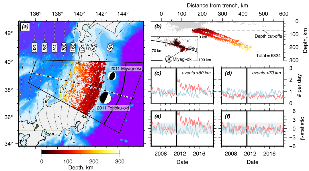
Figure 6. Temporal variations in intermediate-depth seismicity in response to the 2011 M_w 9.1 Tohoku-oki earthquake. (a) Spatial distribution of seismicity used in the analysis from the JMA catalog. Contours of the slab surface are shown as black-dashed lines from Slab 2.0 (Hayes et al., 2018). (b) Cross-section through the seismicity with the two depth cut-offs used in the analysis at 60 and 70 km shown as black dashed lines. Inset is a zoom-in of the seismicity within \pm 1 month of the 7 April 2011 Miyagi-oki earthquake. The aftershocks of the Miyagi-oki earthquake clearly extend 10–15 km below the slab surface, but remain shallower than 70 km depth. (c) Average number of earthquakes per day in the upper plane (light red) and lower plane (light blue) of the double-seismic zone (DSZ) for all events >60 km depth. The time-series is calculated using a sliding window of length 0.2 years and time step 0.05 years. The vertical black line marks the timing of the Tohoku-oki mainshock. (d) Equivalent plot to (c), but for all events >70 km. (e) and (f) show the \beta -statistic of Matthews and Reasenberg (1988) for all events >60 km and >70 km depth, respectively. If \beta exceeds 2, this is equivalent to the earthquake rate deviating more than 2 standard deviations from background, with the background defined by the seismicity rate during the period 2006–2011.
