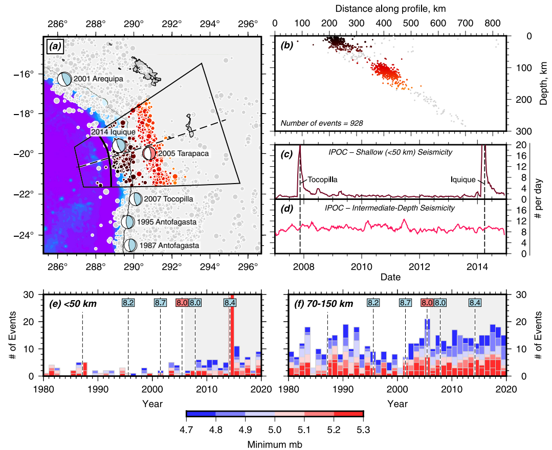
Figure 7. Overview of seismicity in northern Chile between 1980 and 2020. (a) Map view of the distribution of seismicity from the ISC catalog with m_b \geq 4.7 with the focal mechanisms of the largest mainshocks. Gray circles represent earthquake hypocenters, and colored circles represent earthquakes used in the analyses in (b, e, f). Dark colored circles are shallow earthquakes and red-orange colored circles are intermediate-depth earthquakes. (b) Cross-sectional view of the seismicity projected onto the black-dashed path in (a) showing the cluster of seismicity at \sim 400 km distance along the profile. (c) Temporal evolution of shallow ( < 50 km) seismicity in northern Chile from the IPOC catalog of Sippl et al. (2018) calculated using a sliding window of width 0.1 year and time steps of 0.02 years (d) Same as (c), but for the intermediate-depth seismicity between 70 and 300 km depth. (e) and (f) show histograms of the number of earthquakes in the ISC catalog with m_b > M each year for the shallow and intermediate-depth seismicity, respectively. The area in gray marks the installment of the IPOC network in northern Chile in 2006. Vertical dashed lines mark the timing of major earthquakes in the region and their magnitudes, with megathrust events represented by a light blue box and intraslab events by a light red box.
