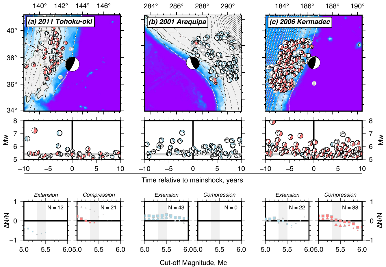
Figure 4. Examples of changes in intermediate-depth earthquake mechanisms before and after three major megathrust earthquakes. Mechanisms are colored red if they are related to down-dip compression, blue for down-dip extension and gray for along-strike deformation. Contours represent the depth to the slab surface from Slab 2.0 (Hayes et al., 2018) and are every 20 km. The middle panel is a time-series of earthquake mechanisms as a function of magnitude. The dark gray horizontal line represents the global magnitude of completeness of the gCMT catalog. The bottom panel shows the difference in the number of earthquakes after and before the megathrust event divided by the total number of earthquakes \Delta N/N = (N_a - N_b)/(N_a + N_b) , for down-dip extensional and compressional events. The vertical gray line shows the range of completeness for the gCMT catalog. Squares and triangles represent \Delta N/N for the period 5 and 10 years either side of the mainshock, respectively. The size of the symbol is scaled by the number of earthquakes in that bin and decreases in size as the number of events in the bin gets smaller.
