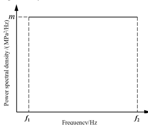
FIGURE 6 Load spectrum of vibration fatigue test
