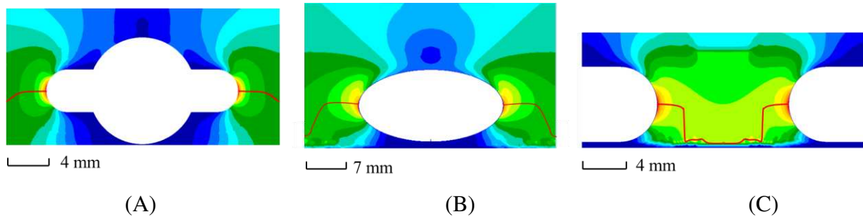
FIGURE 10 Maximum RMS stress line around the notch root (A)central circular hole notched specimen;(B) elliptical hole notched specimen;(C) edge notched specimen.
