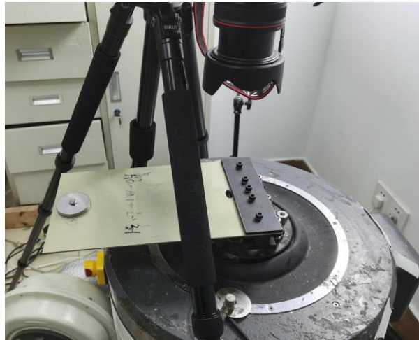
FIGURE 2 Vibration testing site
