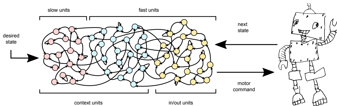
Figure 4: Representing actions via attractor dynamics . Architecture of the model by Yamashita & Tani (2008), in which distinct attractor dynamics in the fast units of a continuous time recurrent neural network come to represent distinct actions performed by a robot, and the dynamics of slower units come to represent configurations of actions. Inputs to the system are proprioceptive signals and visual information about the position of an object to be manipulated. Slow and fast context units are point neuron models with different intrinsic integration time constants. Every unit is connected to every other, including itself, with the exception of input units which do not have a direct connection to the slow context units (an illustrative subset of units and connections is shown for clarity). Activations of the output units are considered to be predictions about future proprioceptive states, and prediction errors are used to adjust the network connection weights using a backpropagation algorithm. Adapted from (69), Figure 3A.
