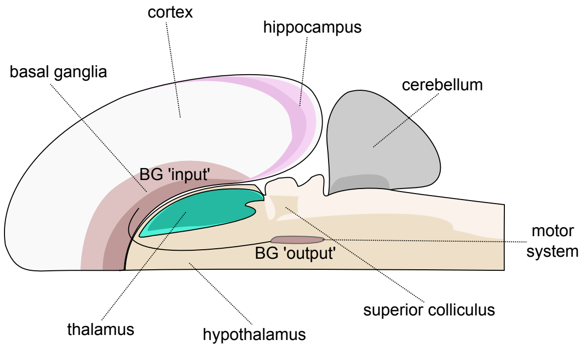
Figure 1: Major functional divisions of the vertebrate brain. ‘Flatmap’ of the rat brain, indicating the overall arrangement of several major functional regions. These have been the targets of some of the computational and neurobotic modelling works discussed in this article.
