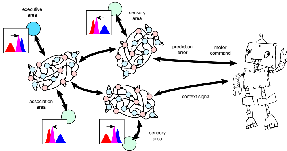
Figure 5: Generating actions to avoid surprise . Architecture diagram based on the study of Idei et al. (54), which demonstrates the emergence of different free energy regimes when proprioceptive and exteroceptive signals provide congruent or incongruent information. The executive area consists of a single latent unit (large blue circle), the association area contains 15 recurrent units (eight fast, blue, and seven slow, red) and three latent units (large green circle, one shown), and the two sensory areas each contain 15 recurrent units and one latent unit. Each recurrent unit in the association area receives weighted inputs from the latent unit in the executive area, from the three latent units in the association area, and from the activation of all recurrent units in the association area at the previous timestep. In a given sensory area, each recurrent unit receives weighted inputs from the three latent units in the association area, from the latent unit in the corresponding sensory area, and from the activation of all recurrent units in that sensory area at the previous timestep. A subset of the recurrent units in each sensory area are assigned as output units and a weighted sum of their activations for each sensor value is interpreted as a prediction of its future state. The predicted proprioceptive states are used as the target values for a PID controller to determine the robot's movements, and the proprioceptive and exteroceptive predictions are continually compared to the actual future states to produce prediction errors. Inset graphs indicate shifts in the latent variables (pink) to minimize free energy.
