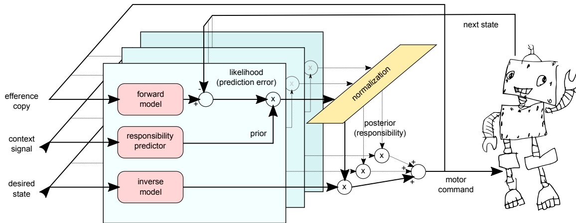
Figure 3: Selecting between control modules . Architecture diagram for the Mosaic model (58). Pairs of forward and inverse models are tuned according to how well their outputs match the future states of the robot. Proprioceptive prediction errors generated by each forward model are weighted by contextual signals from other sensors and then normalized across modules to create a distribution of ‘responsibilities’, which in turn weight the contribution of corresponding inverse models to the overall motor command. Prediction errors, responsibility predictors, and the normalized responsibilities can be considered as likelihood estimations, priors, and posteriors, and as such the model implements a form of the Bayesian belief updating that is used extensively in current predictive processing systems. Based on Haruno et al. (59), Figure 1., omitting notation and an additional feedback controller loop for clarity. ‘Judy the Robot’ drawing by Pippa Wilson.
