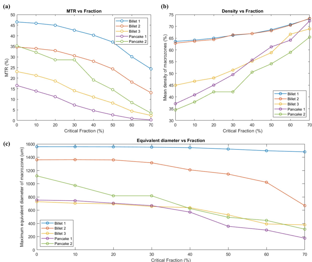
Figure 9 Results from the effect of the critical-fraction criteria in five different data sets on (a) MTR, (b) mean density and (c) maximum equivalent diameter of the macrozone.
