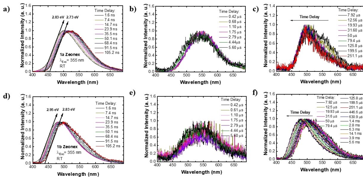
Figure 3. a, b, c) Time resolved normalised emission spectra of 1a and d, e, f) 1b in zeonex matrix. All spectra collected at room temperature under vacuum.
