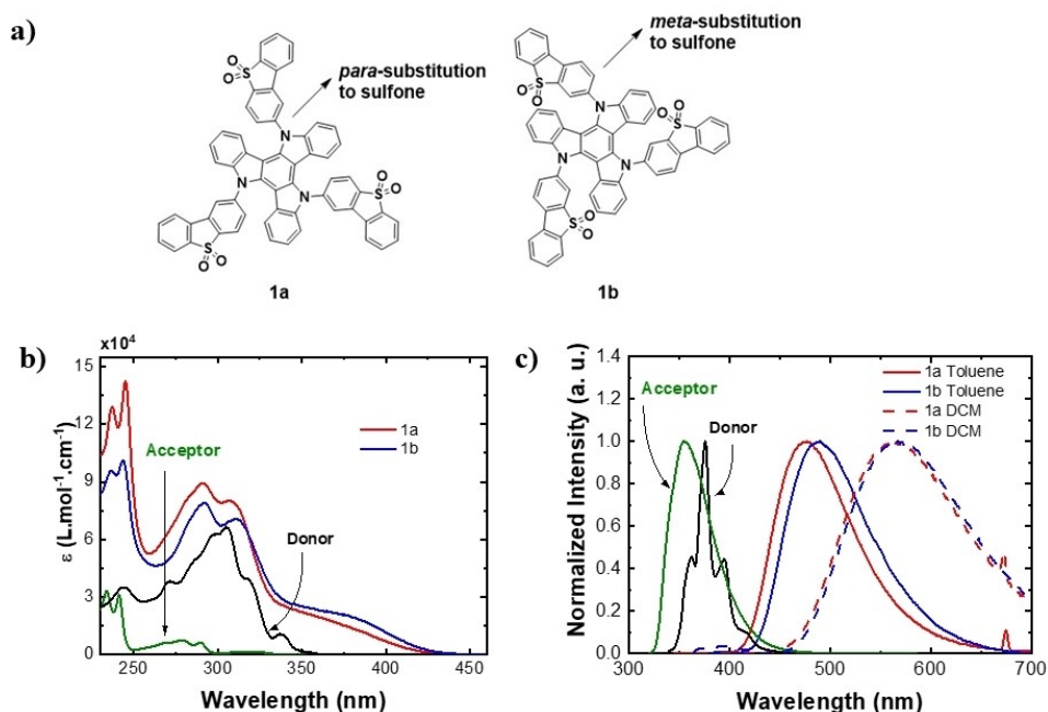
Figure 1. a) Chemical structure of para -substituted emitter ( 1a ) and meta -substituted emitter ( 1b ). b) Extinction coefficient absorption spectra of the acceptor (A), donor (D), 1a and 1b , all diluted in dichloromethane (DCM) solvent. c) Normalised photoluminescence (PL) spectra of A, D, 1a and 1b . D and A are diluted in toluene solvent, 1a and 1b are diluted in toluene and DCM. Data for A, D and 1a are taken from Reference [8].
