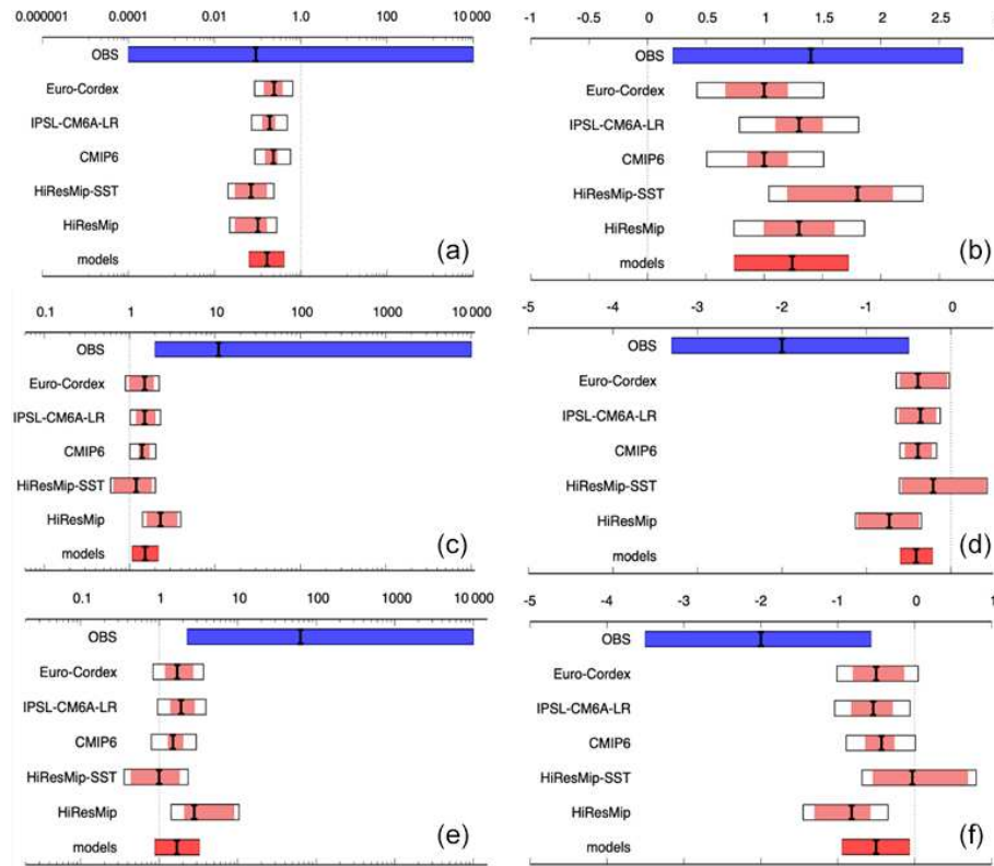
Figure 8. Changes between the past and present: summary of observational (blue) and model (red) results for probability ratio (a, c, e, giving the change in the probabilities between the climate with a 1.2 °C cooler global temperature and the current climate, as well as change in intensity [°C] (b, d, f) in the three indices, TNnApr–Jul (a, b), TNnGDD250 (c, d) and TNnGDD250–350 (e, f), as averaged over the study area (see rectangle in Fig. 2b). Extent of the bars gives the two-sided 95 % confidence intervals accounting for internal variability (pink) of each ensemble and model spread added (white), calculated as explained in Philip et al. (2020), with the black marker indicating the best estimate. A weighted average of model results is shown in bright red (label “models”). Note that, for the index TNnApr–Jul, only EURO-CORDEX and HighResMIP-SST passed the validation step, but other models are included in the weighted average for reasons described in the text.
