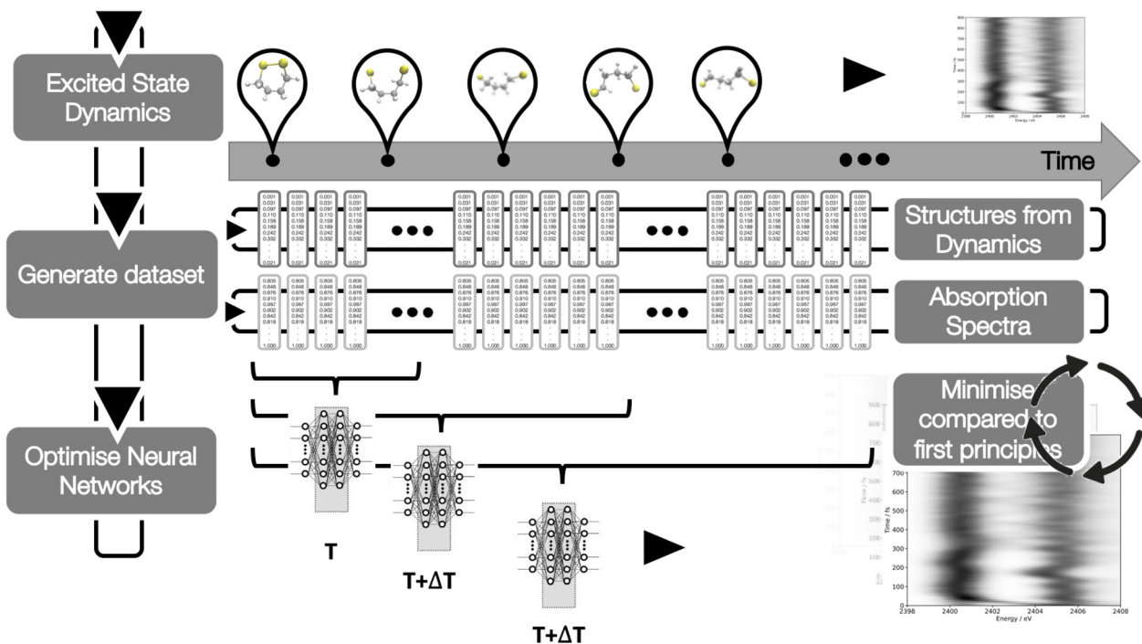
Fig. 2 A schematic of the workflow used in this Article. The DNN takes as input geometries obtained from the TSHD simulations of 1,2-dithiane, carried out in ref. 30, and the calculated sulphur K-edge XAS spectra for these geometries up until some time, T , after excitation. These pairs of geometries and sulphur K-edge XAS spectra constitute the reference dataset on which the DNN carries out supervised learning. The optimised DNN is used to predict the sulphur K-edge XAS spectra for all future timesteps up until the final timestep, and the error – or loss – associated with the predictions is quantified by the cosine similarity between the theoretical target and DNN-predicted sulphur K-edge XAS spectra. This process is repeated at sequential timesteps, T + \Delta T , until the cosine similarity between the theoretical target and DNN-predicted sulphur K-edge XAS spectra converges.
