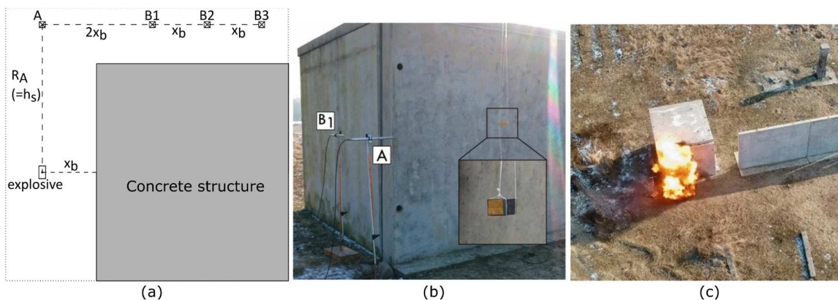
Figure 9. Schematic of the experimental set-up (a) and field test photographs (b,c) used in [11].
