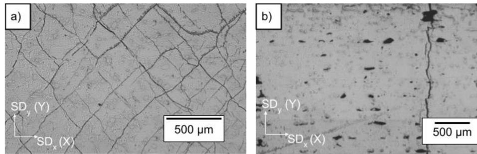
Fig. 6. Optical micrograph of 2_300_B sample (a) XY plane showing that the cracking shows a distinct pattern with the cracks running in preferred directions of 45^\circ and 135^\circ to the X axis. As there are a large number of cracks, it would be unsuitable to infer the crack distribution throughout the whole sample using only one micrograph. Sample 5_800_B (b) showing both cracking and LOF defects.
