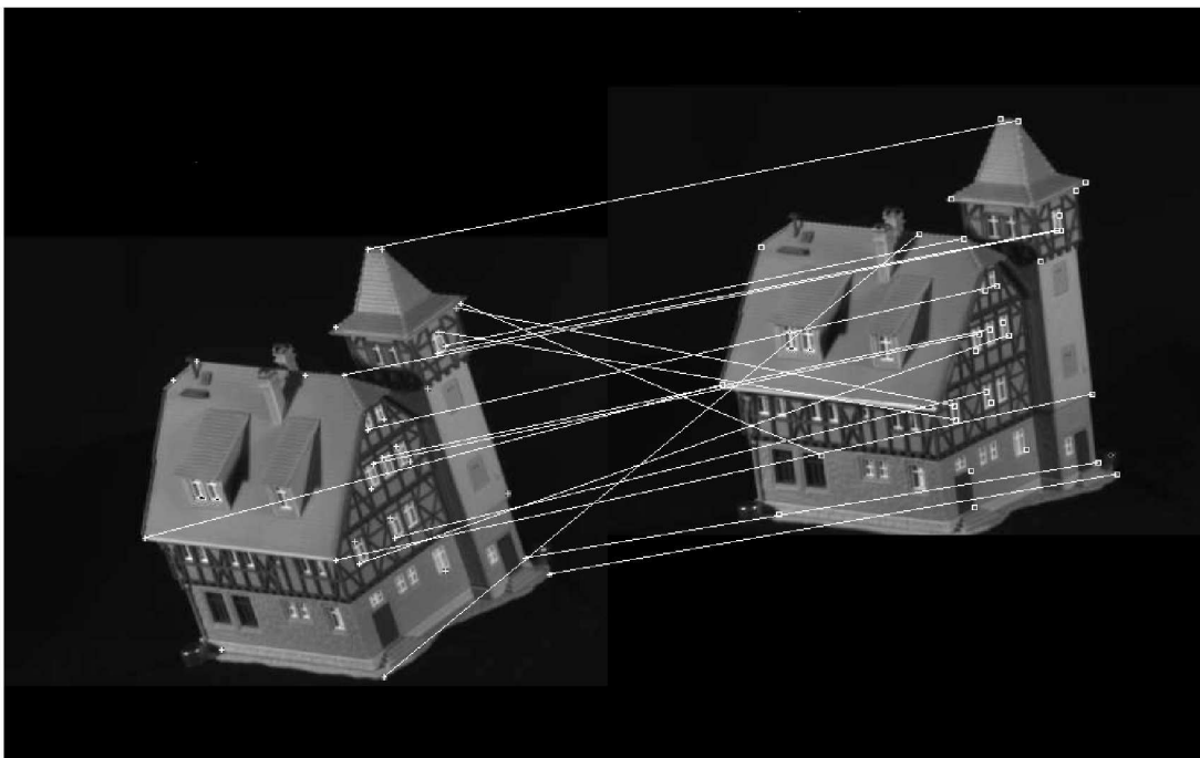
Fig. 14. Correspondences from the Umeyama algorithm.
