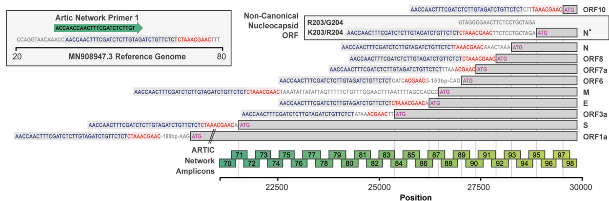
Figure 3. The configuration of canonical sgRNAs and the novel non-canonical nucleocapsid sgRNA (N * ) in SARS-CoV-2. The bottom bar illustrates the presence of the leader sequence (blue text) followed by the transcription-regulating sequence (TRS; red text) within the genomic sequence that continues into the first ORF 1a. The presence of other canonical sgRNA transcripts in which the leader sequence and TRS precede the start codon (methionine; pink) of the other proteins are shown. The presence of the novel non-canonical sgRNA transcript containing the K203/R204 polymorphisms (N * ) is shown. The ARTIC primer locations and resultant amplicons are shown.
