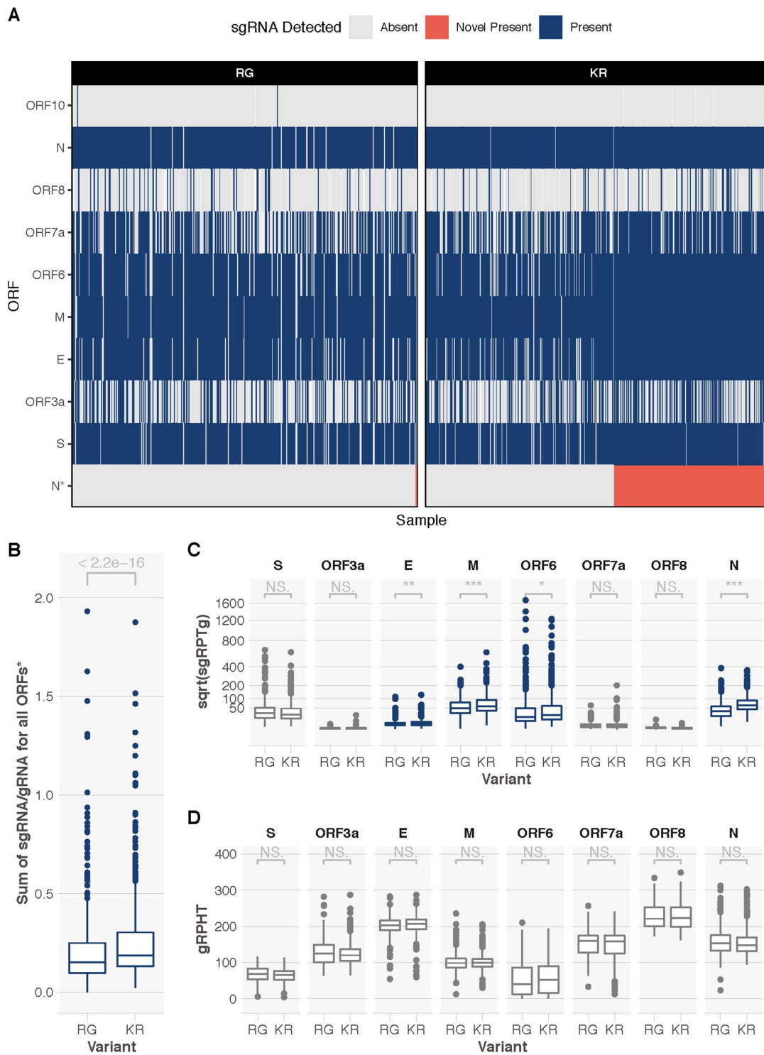
Figure 4. Exploration of sgRNAs in 981 samples from Sheffield, United Kingdom. A. A heatmap showing presence or absence of sgRNAs from different ORFs. K203/R204 (KR)-containing sequences have evidence of the novel truncated N ORF sgRNA (N*, red, 233/553, 42%). An ORF sgRNA was deemed present if we could find \geq 1 read in support. Heatmap is ordered by the presence or absence of the novel
