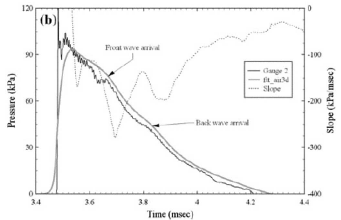
Figure 2 Comparison of measured (Gauge 2) and numerical (FTT_AIR3D) pressure histories for the 15° obliquity target and differentiation of numerical results (Figure 4b in Rose et al. )
