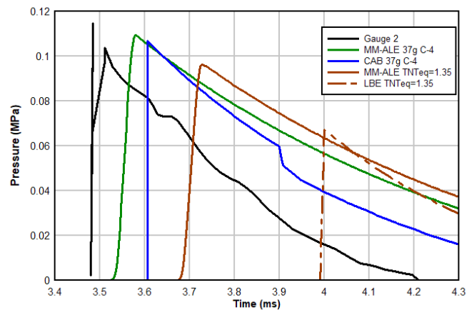
Figure 15 Comparison of pressure history at Gauge 2 with MM-ALE and LBE results for TNTeq=1.35 and MM-ALE and CAB results for 37 g C4
