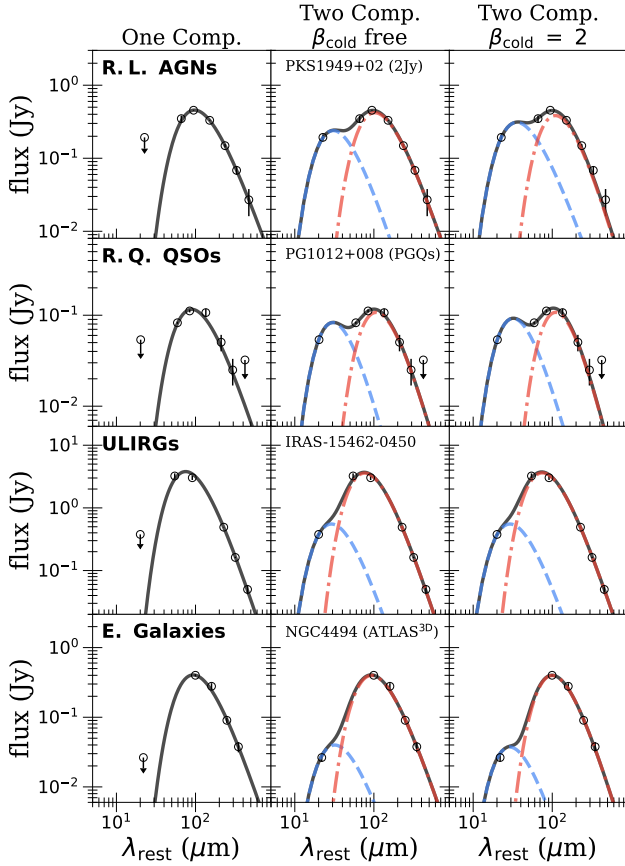
Figure 1. Examples of SED fits for one objects of each of our populations of galaxies. From top-to-bottom, these are radio-loud AGNs, radio-quiet QSOs, ULIRGs, and non-AGN elliptical galaxies, as indicated in the top-left corner of each of the leftmost panels. The names of the sources and their respective samples selected to illustrate our SED fits are indicated at the top of each of the central panels. From left-to-right, the panels correspond to each of our three different models for the dust emission as described in §3.1.1. The observed fluxes are shown with open circles, and the best SED fits with a continuous black line. Downward arrows indicate upper limits on the fluxes. The warmer and the colder dust contributions are shown with a dashed blue line, and a dot-dashed red line, respectively, for corresponding models. 13
