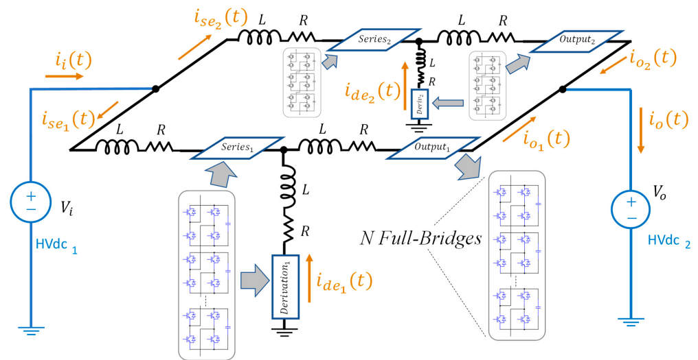
Figure 3. Scheme of the double-T topology.
