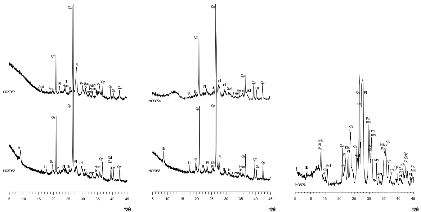
Figure 9. Examples of diffractograms of different PXRD fabrics. Bottom left: MOS062, fabric CGTOS-I. Top left: MOS067, fabric CGVEL-MAG-III. Bottom middle: MOS068, fabric CG17-I; top middle: MOS054, fabric CG19-I; right: loner CGMOS051. And: andalusite; Anl: analcime; Adr: andradite; Cal: calcite; Hem: hematite; Illt: illite-moscovite; Kfs: K-feldspar; Pl: plagioclase; Px: pyroxene; Qz: quartz; Spl: spinel; Sps: spessartine. Abbreviations after [59] (except for Px).
