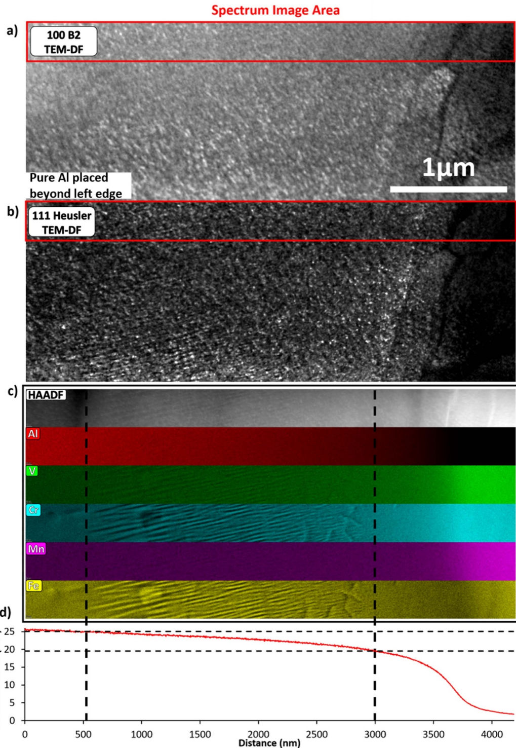
Figure 9. TEM-dark fields (DFs) across the medium–low Al boundary, using a B2 (100) type (a) and a Heusler (111) type (b) reflection. (c) STEM-HAADF and EDX elemental maps of the red region. (d) shows the quantified Al content across this region. The two phase region can be seen to occur between Al contents of 19.5–25 at%.
