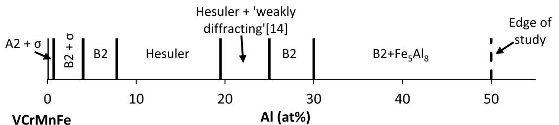
Figure 13. Partial empirical phase diagram of VCrMnFe–Al measured following heat treatment of 800 °C for 240 h followed by 600 °C for 240 h. The dotted line is not the end of the phase field, rather the end of the data presented in this paper.
