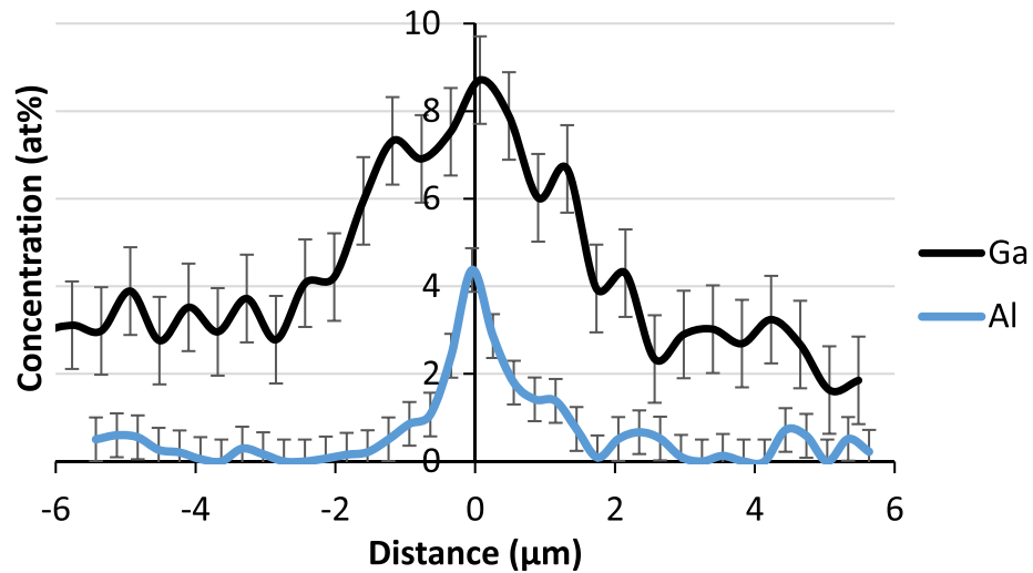
Figure 11. SEM-EDX line profiles across grain boundaries in regions of VCrMnFe + Ga and Al, near where sigma phase begins to form.
