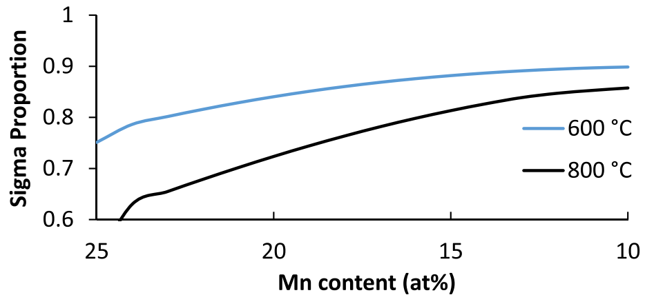
Figure 12. Proportion of Sigma phase in VCrMnFe at 600 and 800 °C, with the Mn content varied along the x axis. Calculated using Thermocalc's HEA4 database.
