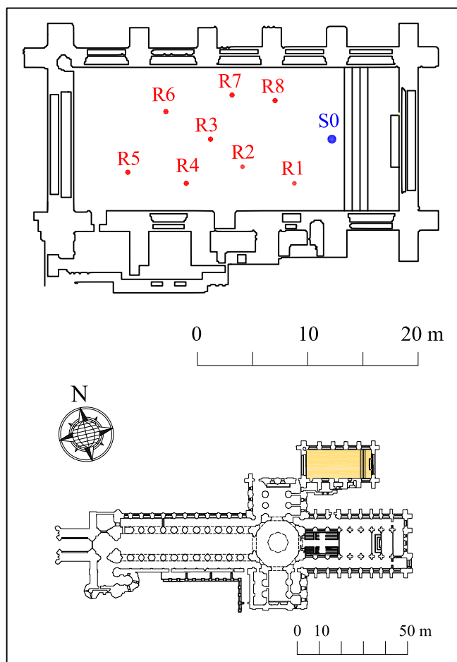
Fig. 1. Sketches of Ely Cathedral's Lady Chapel floor plan, with the sound source (S) and receiver (R) locations set for the measurement session (upper row) and the Lady Chapel's location in the cathedral floor plan (highlighted in yellow).
