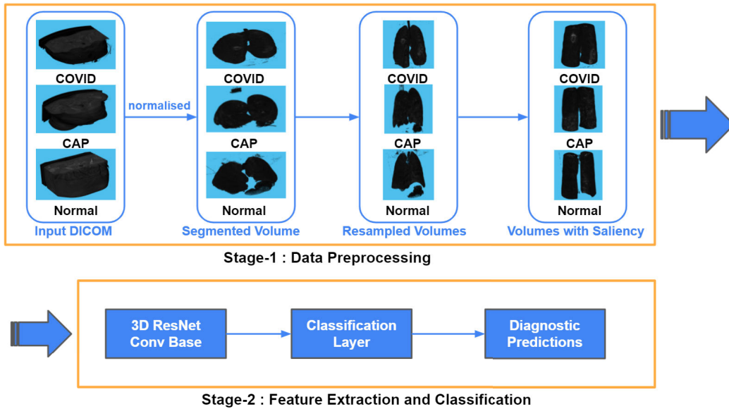
FIGURE 2. An overview of the 2-stage pipeline of our proposed method. Stage-1 includes data pre-processing while stage 2 includes feature extraction and training/classification.
