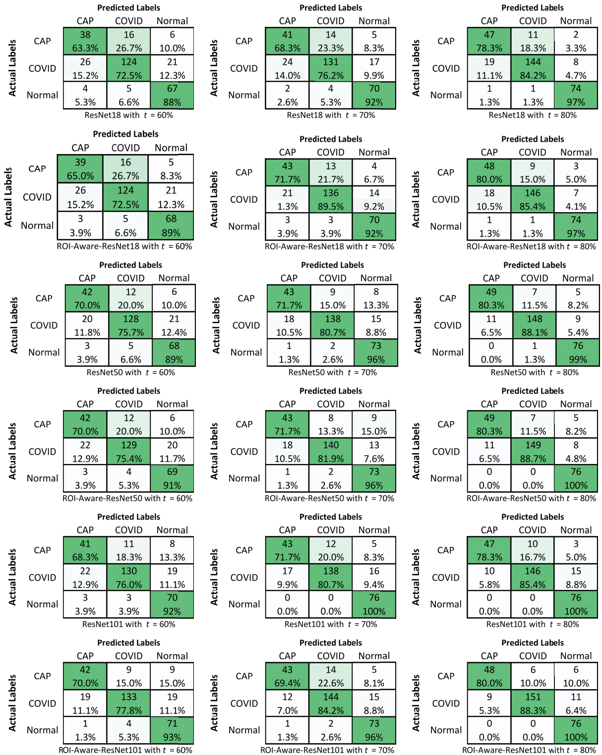
FIGURE 8. Confusion Matrices showing model performance using 5-fold cross validation for various saliency threshold values ( t = 60\% , t = 70\% and t = 80\% in columns 1-3, respectively), for different 3D networks (3D ResNet-18, 3D ResNet-50 and 3D ResNet-101, in rows 1,3 and 5 respectively) and their RoI-Aware modified versions (the proposed method) in rows 2, 4 and 6, respectively.
