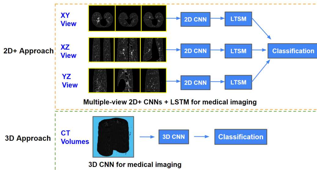
FIGURE 1. Comparison between 2D+ and 3D CNN for medical images classification.
