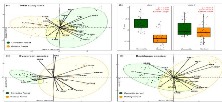
FIGURE 2. Principal component analysis (PCA) showing the distribution of functional traits vectors of cerradão and gallery forest (a). Axes with statistical differences by Mann-Whitney test (b). PCA by species subgroups considering leaf deciduousness (c) and (d). More details on the factorial load of the traits per axis – Appendix S2 (see the Supplementary Data with this article). PCAs by Forest and statistical difference by subgroups considering deciduousness – Appendix S3.
