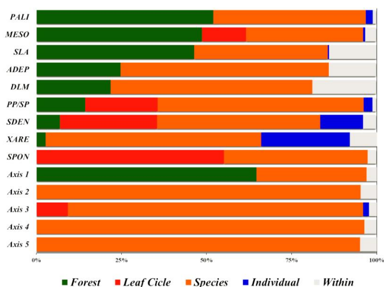
FIGURE 6. Partitioning the variance of nested linear mixed models of the functional traits of two tree communities in the Amazon-Cerrado transition. Specific leaf area (SLA), palisade parenchyma thickness (PALI), leaf blade mesophyll thickness (MESO), adaxial epidermis thickness (ADEP), palisade parenchyma thickness (PP-SP), spongy parenchyma thickness (SPON), average lumen area of xylem vessels (XARE) and axes of the PCA. Within means the residual error, all data were transformed (log-10) before analysis.
