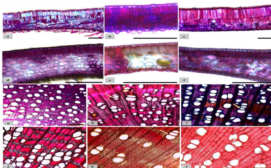
FIGURE 5. Cross sections of leaves (A-F) and young branches (G-L) of dominant species from tree communities of two Cerrado forest formations. Cerradão dominants' leaves: trichomes in Emmotum nitens (A), thick epidermis in Pterodon pubescens (B), thick cuticle in Pouteria ramiflora (C); Gallery forest leaves, with dorsiventral mesophyll and showing much greater spacing in the spongy parenchyma: Aspidosperma subincanum (D), Ephedranthus parviflorus (E) and Unonopsis guatteroides (F). Cerradão plants with higher vessel density and smaller vessel diameter (G - Myrcia splendens , H - Tachigali vulgaris and I - Mezilaurus crassiramea ); Gallery forest plants with lower vessel density and larger vessel diameter (J - Pouteria gardneri , K - Apuleia leiocarpa and L - Mabea pohliana ). Bars: 150 \mu m (A-F), 200 \mu m (G-L).
