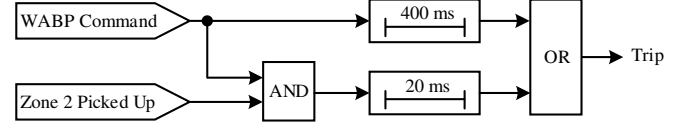
Fig. 5. Tripping logic of the proposed method.
