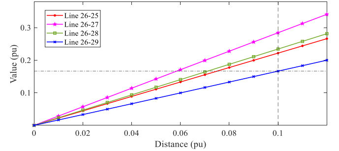
Fig. 9. Mismatch degree between the coefficient vector at bus 26 and the coefficient vectors at distance 0 to 0.12 pu on all lines connected to bus 26.
