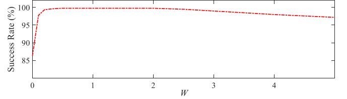
Fig. 8. Sensitivity of the proposed method to the value of W .
