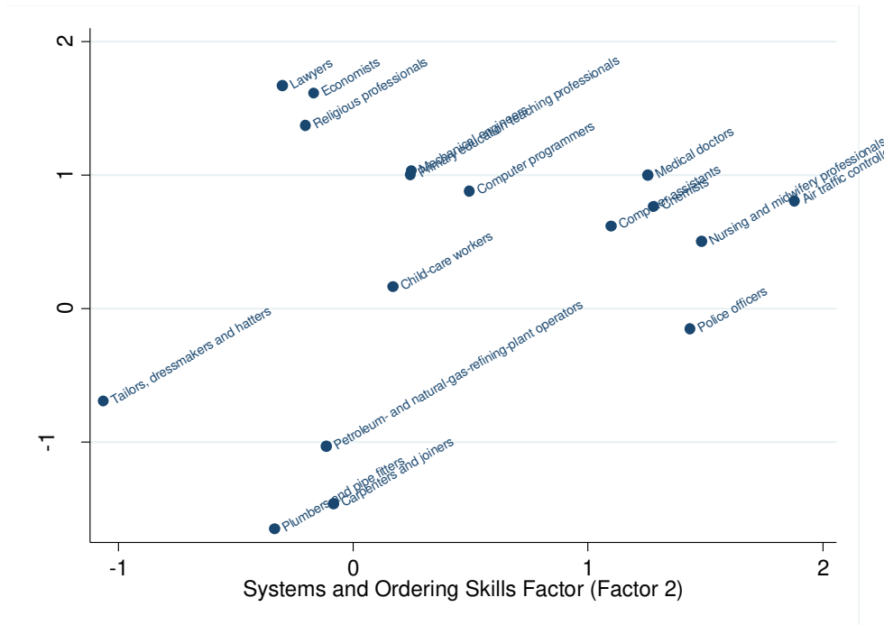
Figure 1: Factor Scores for Selected ISCO-88 Occupations
