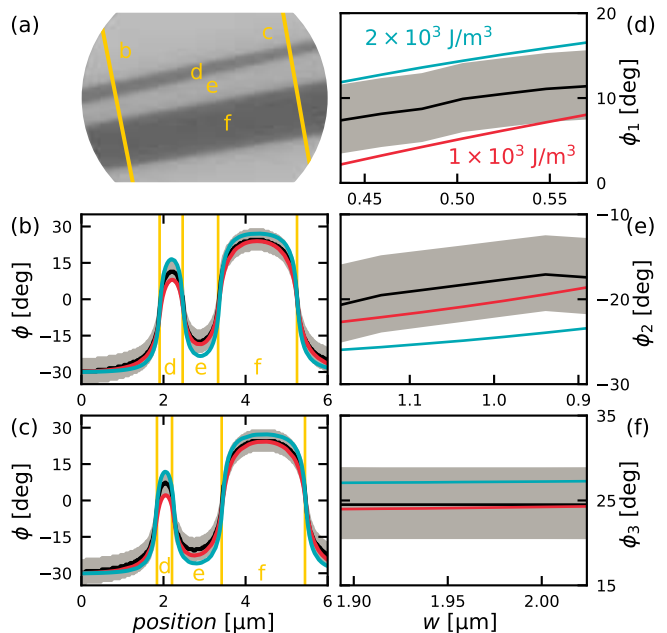
FIG. 4. Determination of the anisotropy constant: (a) Fit to the image in Figure 1(c), as described in the main text. (b) & (c) Profiles of the magnetization angle along the corresponding yellow lines in panel (a). The experimental data (black lines with gray shading indicating the uncertainty) is compared to micromagnetic simulations for a uniaxial anisotropy of K_u = 1 \times 10^3 and 2 \times 10^3 J/m 3 (red and turquoise lines). (d) – (f) Magnetization angle \phi at the center of the three central domains, labelled with the corresponding letter in panel (a), as a function of domain width w .
