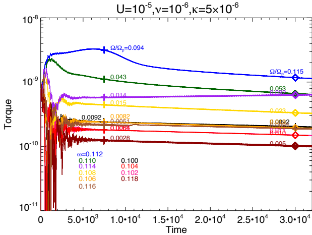
Figure 7. Specific torque versus time for the same simulations as in Fig. 5. The azimuthally averaged angular velocities \bar{\Omega} measured at the centre are labelled in units of the angular pattern speed \Omega_p for t = 7500 (crosses) and t = 30050 (diamonds).
