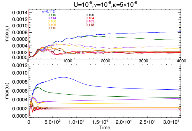
Figure 5. u_{r,\max} versus time for simulations with low-amplitude forcing, Pr = 0.2 , and different forcing frequencies ranging from \omega = 0.100 to \omega = 0.118 with a step size of \Delta\omega = 0.002 . The bottom panel shows the same cases as the top panel but for longer times.
