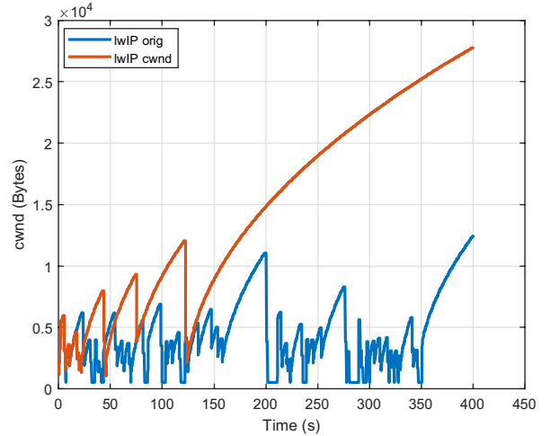
Fig. 3: Congestion window progress of lwIP and lwIP_cwnd algorithms.
