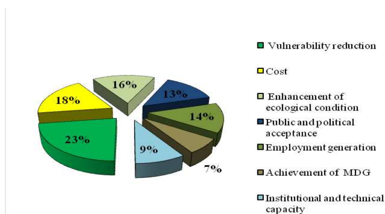
Figure 15: Criteria weights
