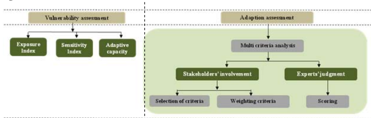
Figure 8: Assessment framework
