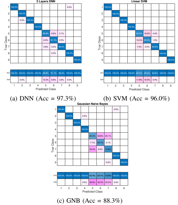
Fig. 2: Confusion matrices for various types of models. N = 50 parameters/sample.
