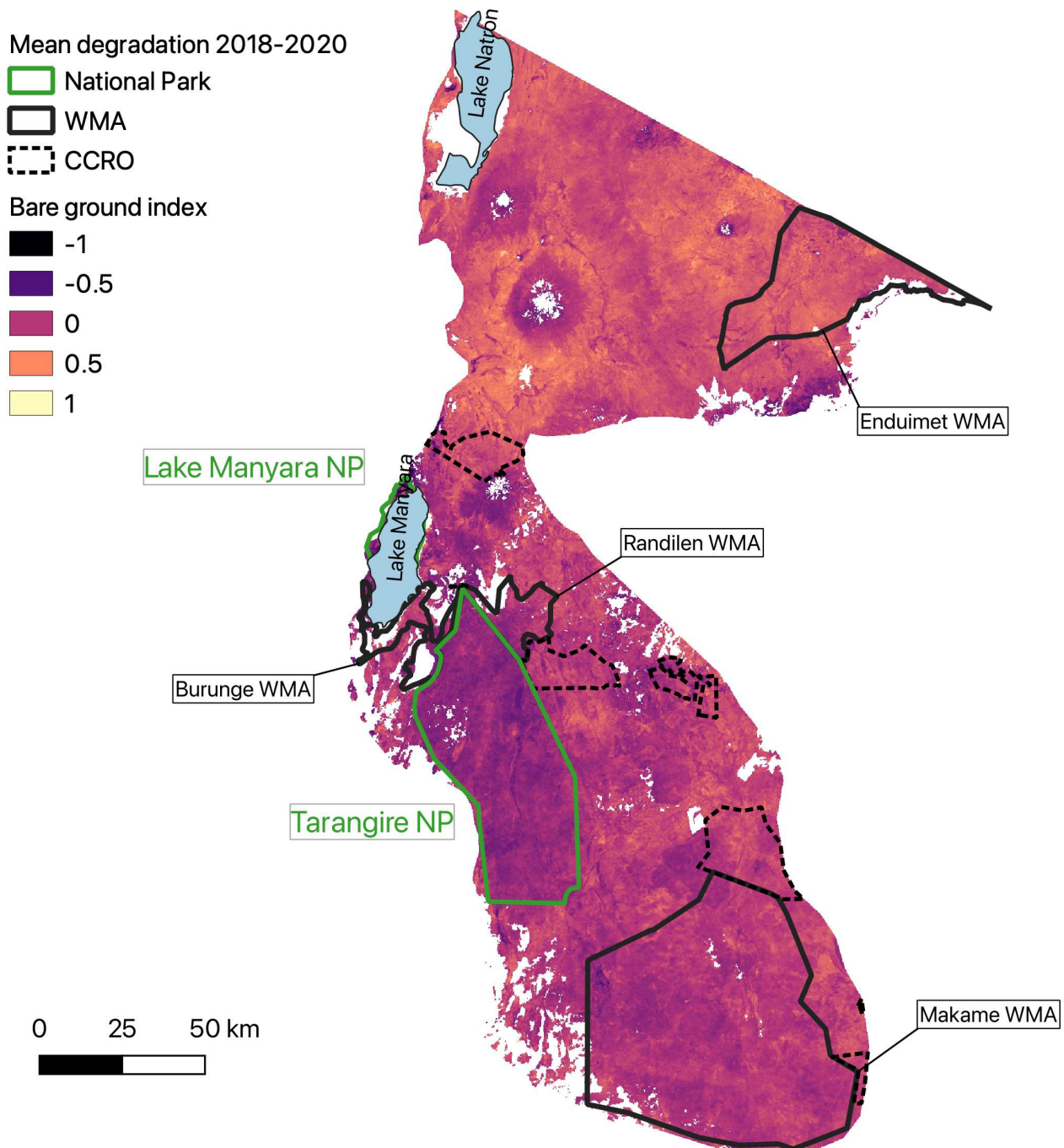
Figure 3. Map of normalized bare ground index scores in the study area, averaged for the years 2018–2020. Areas of high bare ground cover receive higher scores (max index = 1) and are coloured yellow, areas of low bare ground cover have lower scores (max index = -1) and are coloured purple. Gaps in the data (coloured white) are areas removed by the masking layer. The map was created using QGIS 3.14 49 .
