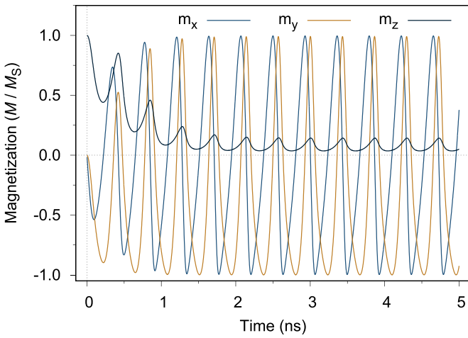
Figure 6. Plot of the dynamic behaviour of a spin-torque nano-oscillator device subjected to a spin-transfer-relaxation-torque of B_{RT}^{STT} = -0.05T , spin-torque asymmetry \lambda = 0.5 , Gilbert damping \alpha_G = 0.01 and external applied magnetic field B_z = 0.01T to break the longitudinal symmetry. The magnetization relaxes from the initial direction \mathbf{m} \parallel z to a dynamic equilibrium after approximately 2 ns where a continuous oscillation is found.
