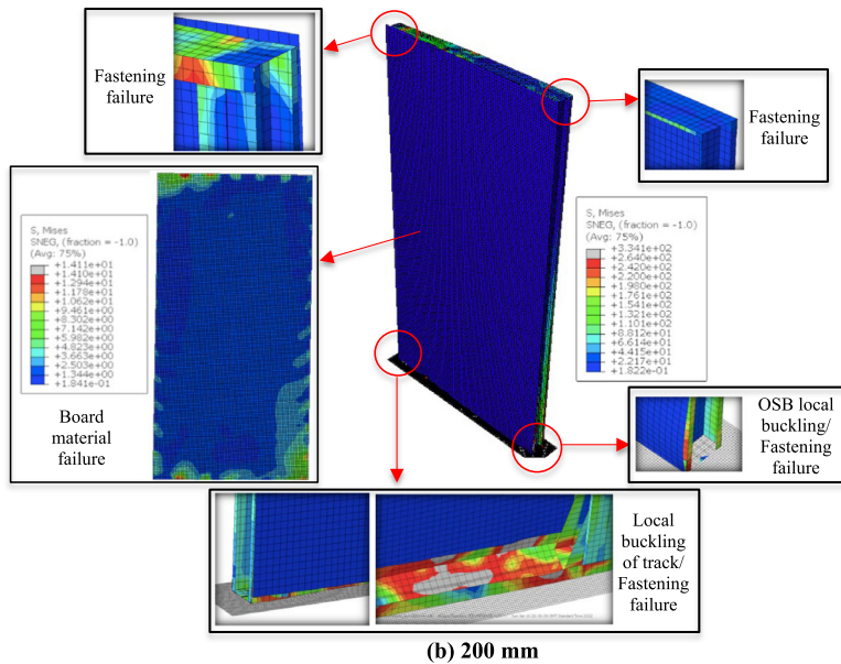
Fig. 14. Von Mises stress distributions in OSB-sheathed CFS wall panels with different screw spacing at failure.
