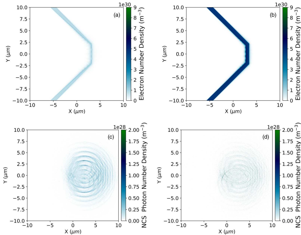
FIG. 1. (a), (b) Electron-density distribution for cone target Al (top left) and Au (top right) at t = 0.2 ps. (c), (d) Photon (NCS) density distribution for cone target Al (bottom left) and Au (bottom right) at t = 75 fs
