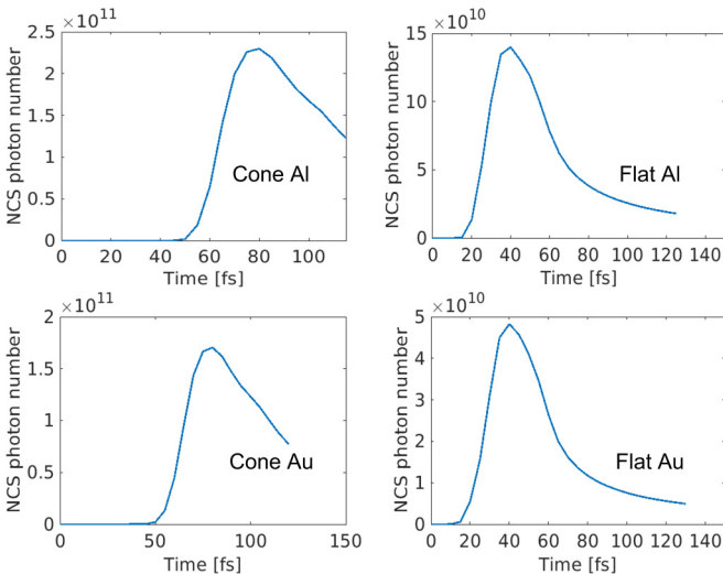
FIG. 7. The photon number in NCS emission for flat and cone Al and Au targets.
