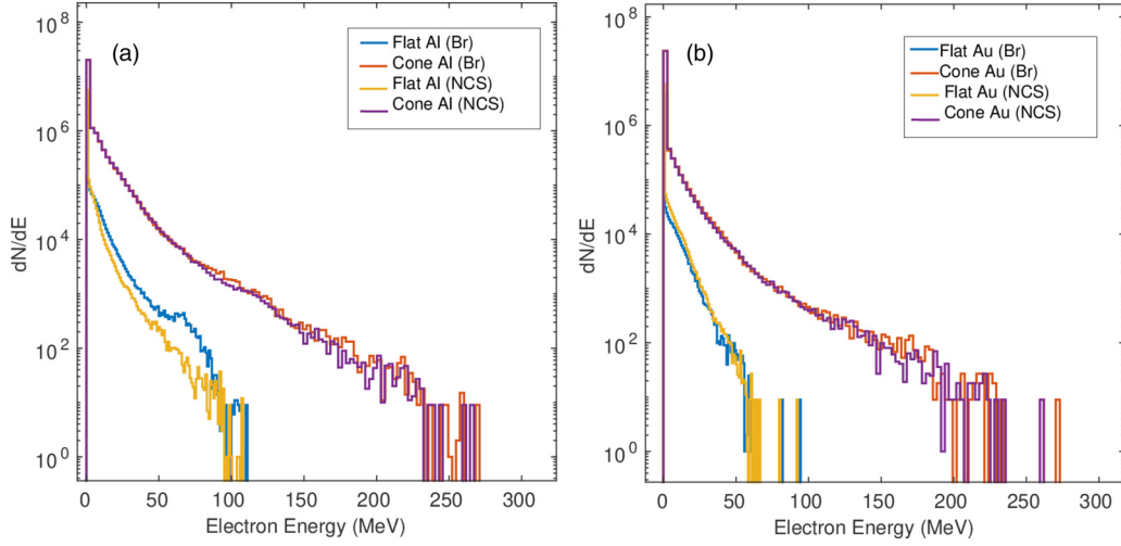
FIG. 3. (a), (b) Electron energy spectra of Al and Au for flat and cone-shaped configuration for the bremsstrahlung and NCS processes.
