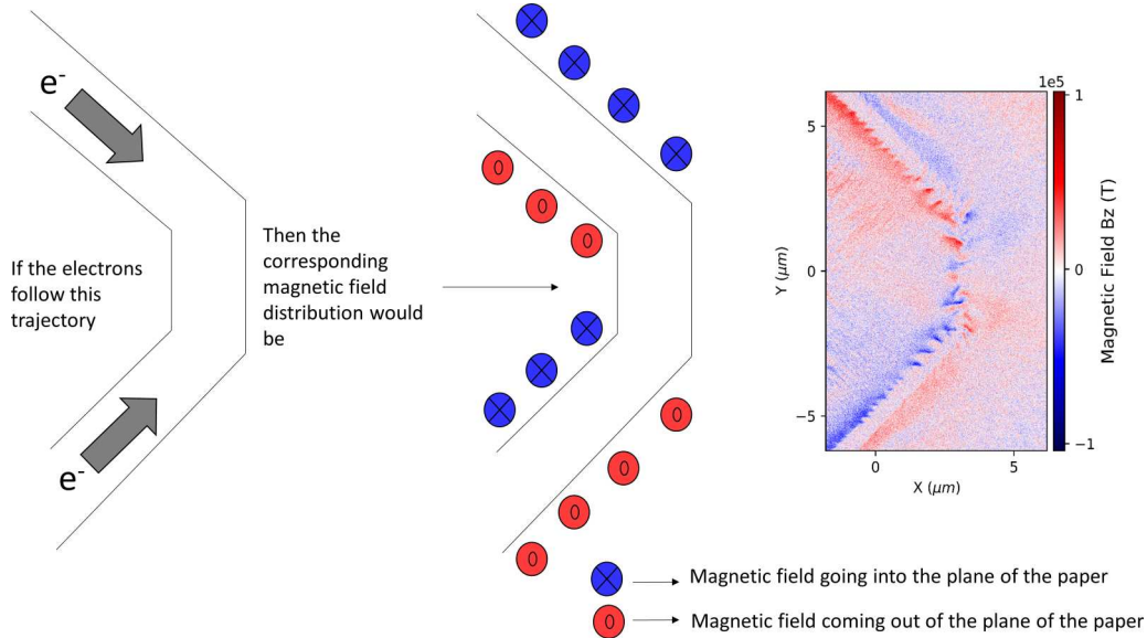
FIG. 11. Tracing of charged particles with directionality of magnetic fields at t = 0.15 ps.
