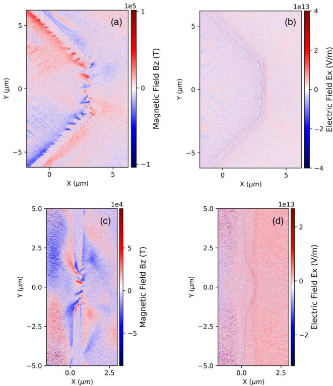
FIG. 8. (a), (b) Magnetic-field (top left) and electric-field (top right) targets for cone-shaped targets at t = 0.15 ps. (c), (d) Magnetic-field (bottom left) and electric-field (bottom right) targets for flat targets at t = 0.115 ps.
