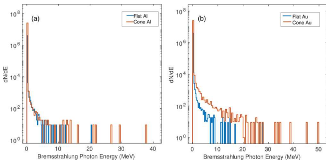
FIG. 4. (a), (b) Photon energy spectra of Al and Au for flat and cone-shaped configuration for the bremsstrahlung process.
