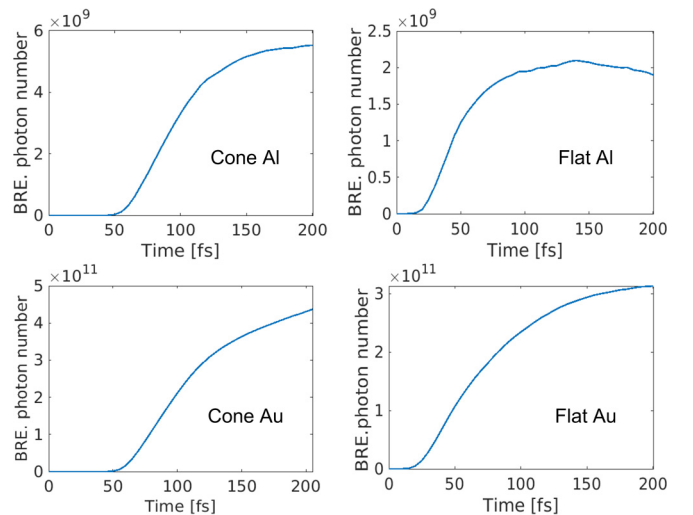
FIG. 5. Photon number in bremsstrahlung emission for flat and cone Al and Au targets.
