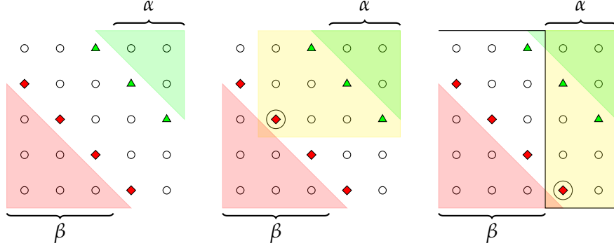
FIGURE 1. With k = 5 , \beta = 3 and \alpha = 2 , one of the red diamond vertices must lie above the staircase (not drawn), and one of the green triangle vertices must lie below. If one of the inner diamond vertices lies above the staircase, the second picture shows all the triangle vertices must also lie above. The last picture shows choosing one of the outer ones leaves one triangle vertex that may lie below.
