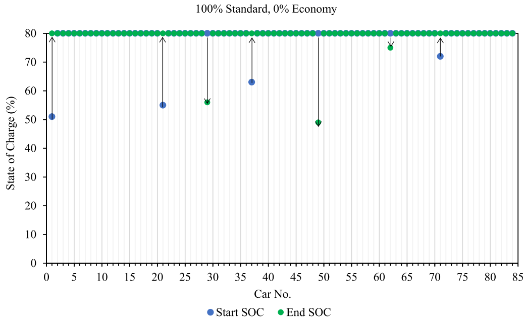
Fig. 10. Start and End SOC's for scenario 8 (100% Standard tariffs).
