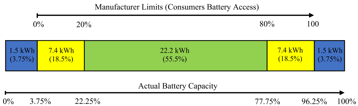
Fig. 2. Battery Capacity (*Not to Scale).
