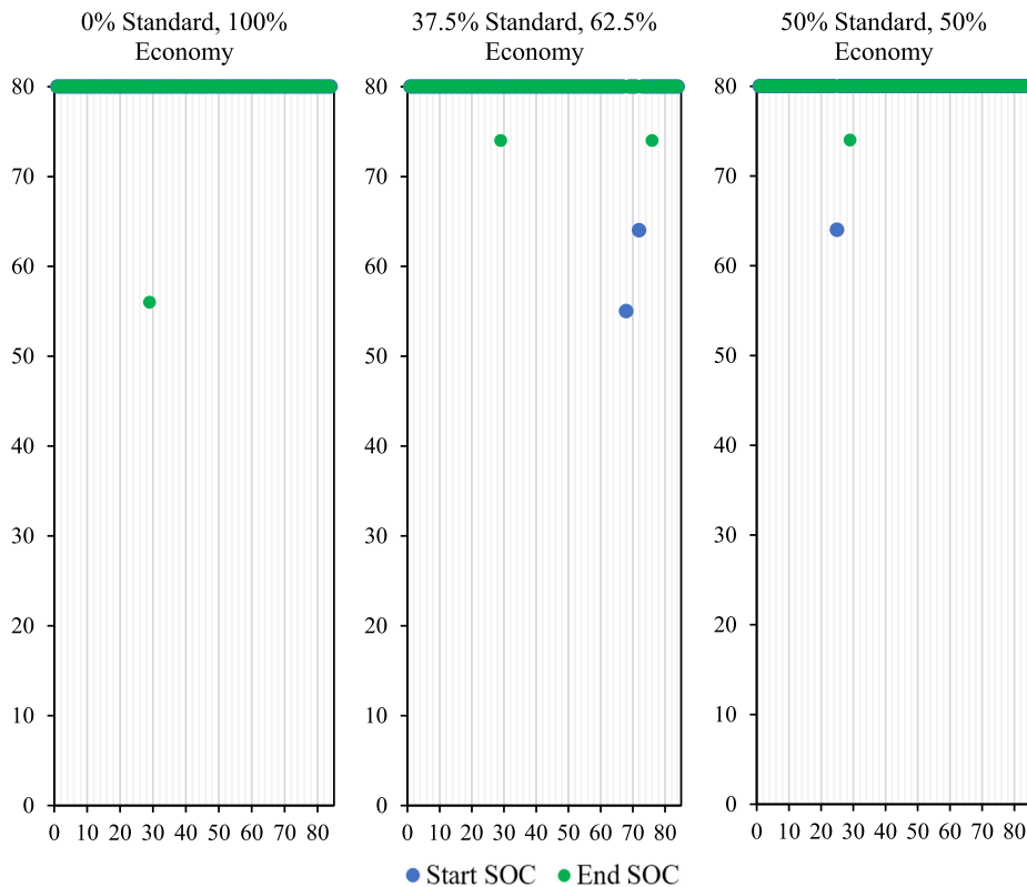
Fig. 11. Start and End SOC's for scenarios 5, 6 and 7.
