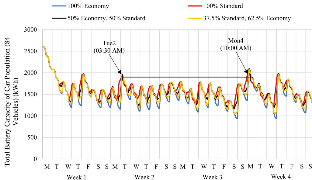
Fig. 4. Total Battery Capacity for the vehicle population of Bradbourne (Scenarios 1, 2, 3 and 4).
