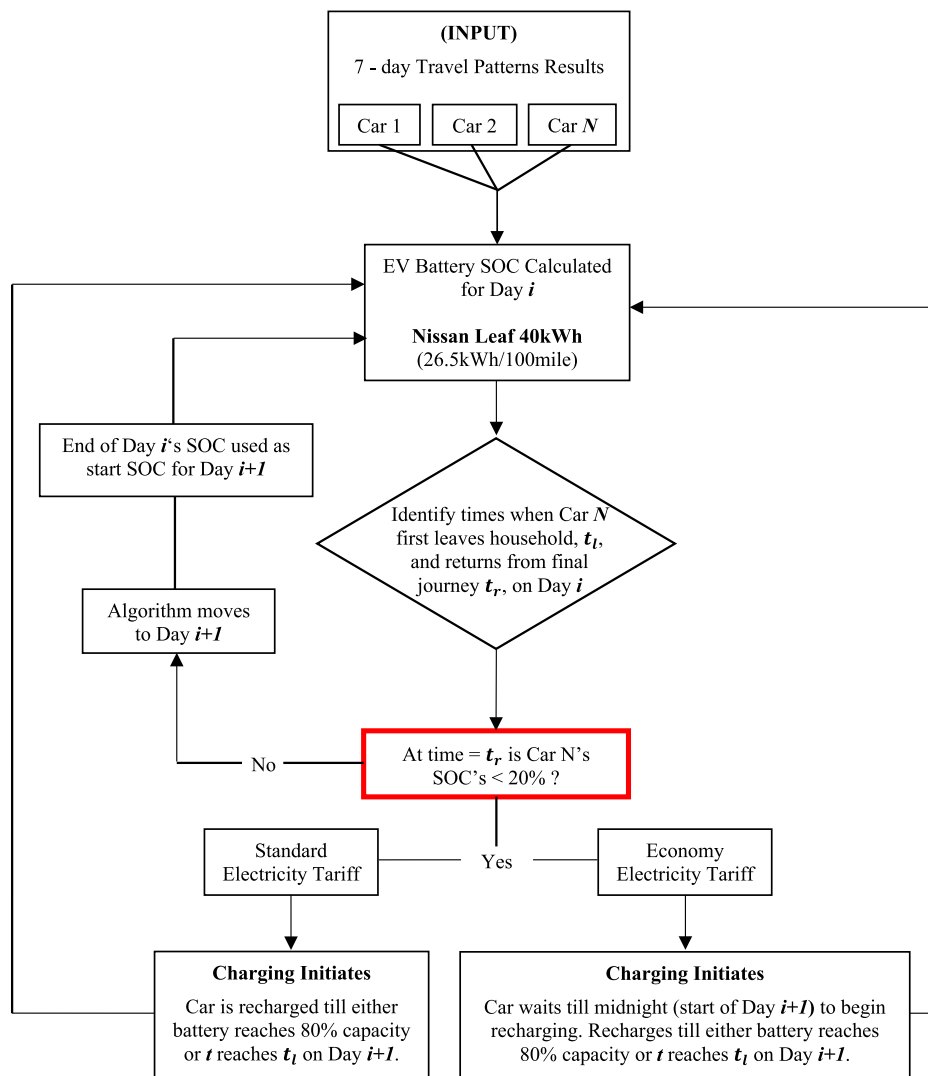
Fig. 3. Flowchart representing the Simulation Process (Charging Initiated when SoC < 20% Scenario).
