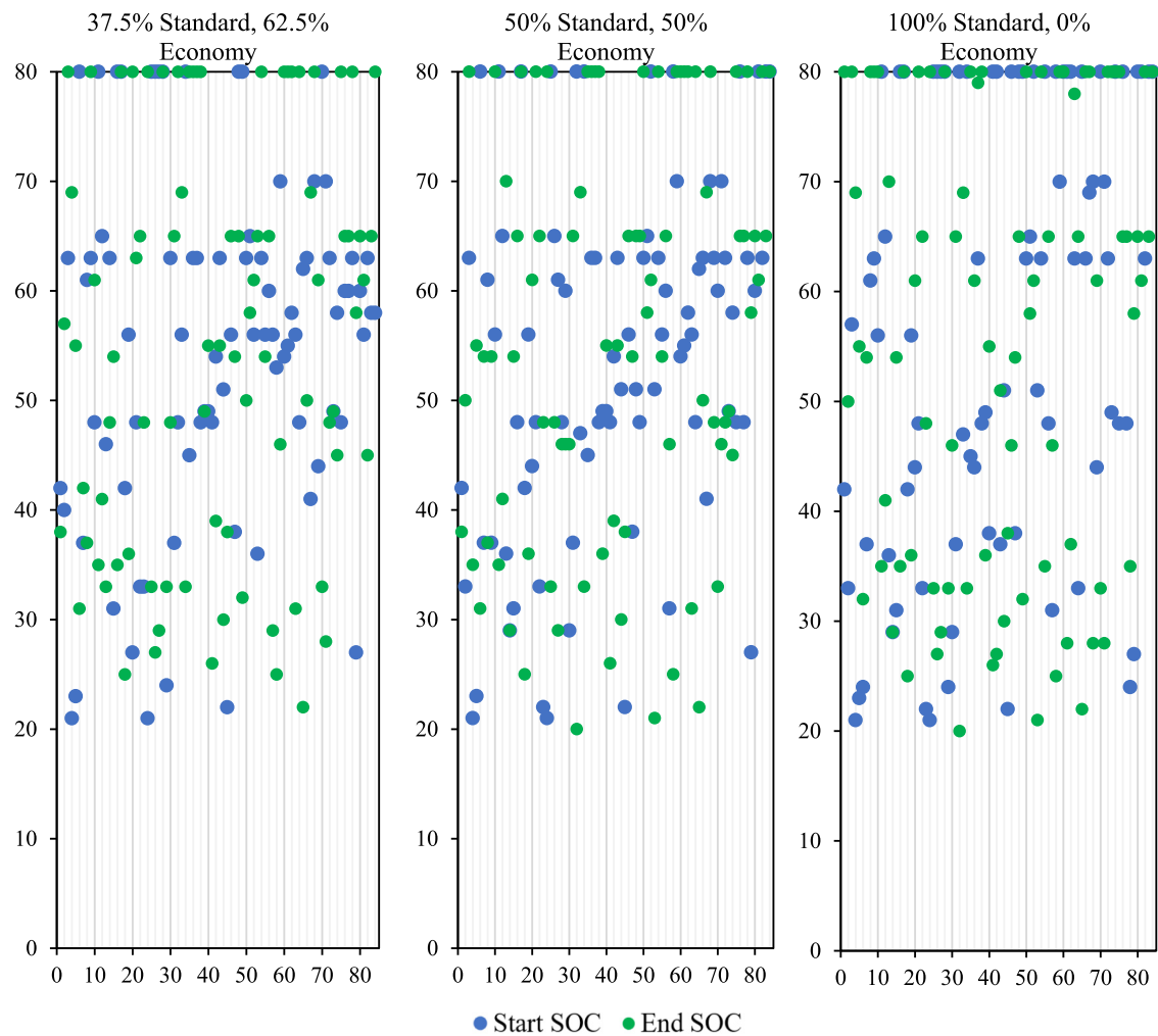
Fig. 8. Start and End SOC's for scenarios 2, 3 and 4.
