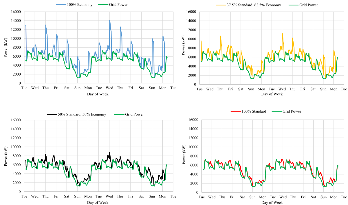
Fig. 12. Grid Impact for Scenarios 1, 2, 3 & 4.
