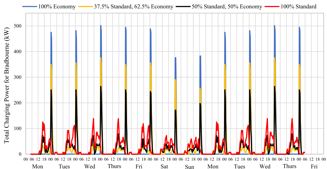
Fig. 9. Charging Power for scenarios 5, 6, 7 and 8.
