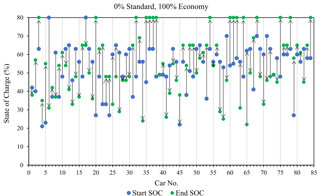
Fig. 7. Start and End SOC's for scenario 1 (100% Economy tariffs).
