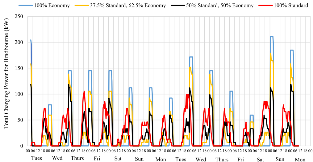
Fig. 6. Charging Power for scenarios 1, 2, 3 and 4.
