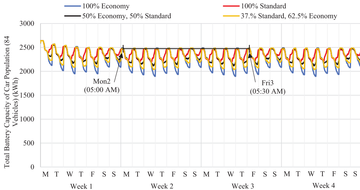
Fig. 5. Total Battery Capacity for the vehicle population of Bradbourne (Scenarios 5, 6, 7 and 8).
