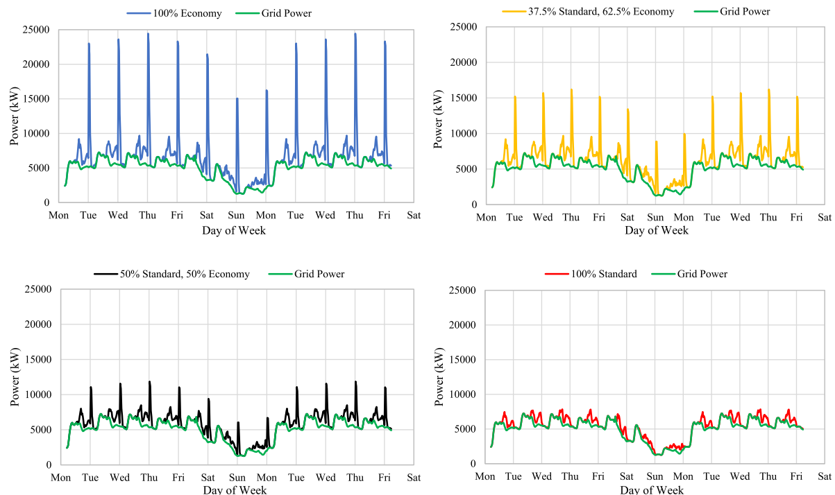
Fig. 13. Grid Impact for Scenarios 5, 6, 7 & 8.
