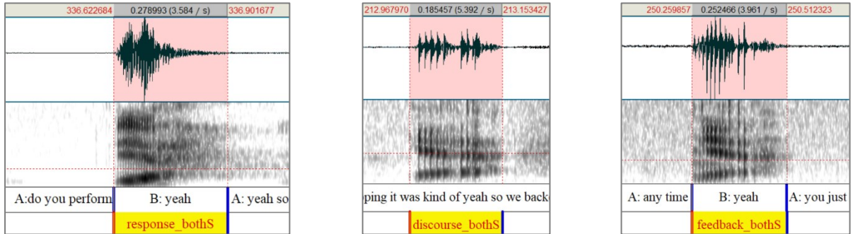
Figure 3: Spectrograms of yeah tokens with different functions: response (left), discourse (mid) and feedback (right).
