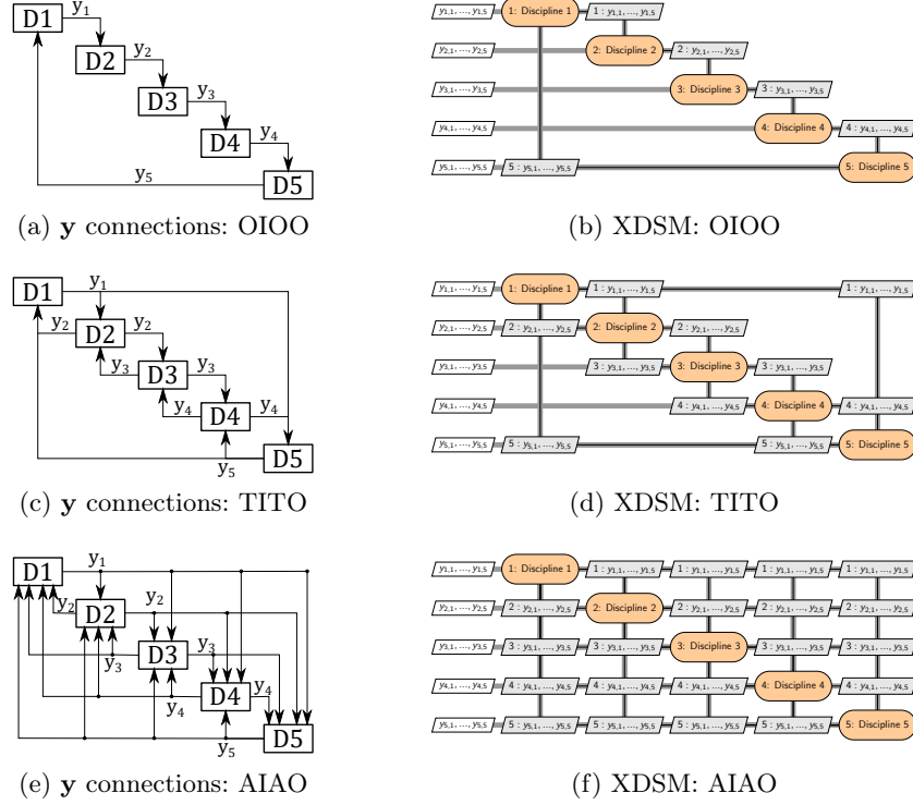
Fig. 1: Different topologies showcasing the dependencies between disciplines on a five-discipline system.
