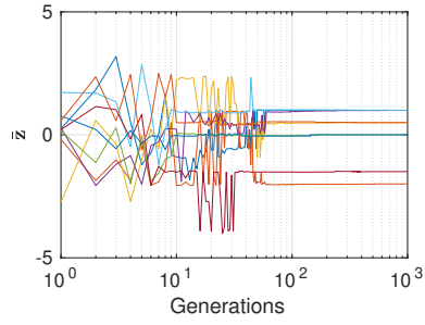
(e) ZDT4-MDO AIAO: globals
