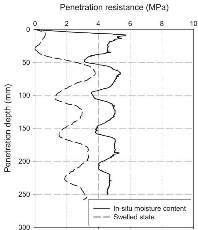
Fig. 8. Measured penetration resistances before and after swell.
