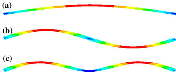
Fig. 4 The first (a), second (b) and third (c) mode shapes of the beam with concentrated middle mass calculated via FE
