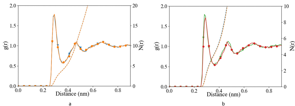
Fig. 2 Radial distribution function (after B-spline interpolation) (left axis) and corresponding integral ( N(r) ) (right axis) between O carboxylate and O w , after 10 ns of classical MD (a) L-Asp, Set_3 unmodified (orange; ●), Set_3 \sigma+0.5\%\sigma (blue; ▼), and (b) glutamic acid, Set_3 unmodified (red; ●), Set_3 \sigma+0.5\%\sigma (green; ▼) when Ca-O carboxylate were in CIP state.
